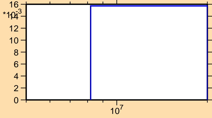
\sigma vs. E for ^{228}\text{Pa}(n,3n)
