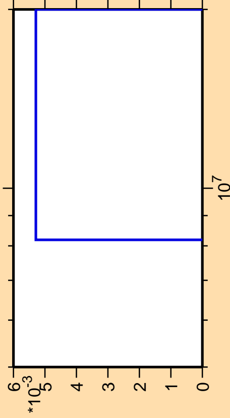
\Delta\sigma/\sigma vs. E for ^{230}\text{Pa} (mt 34)
