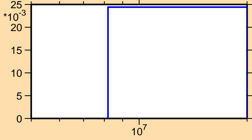
\sigma vs. E for ^{230}\text{Pa}(n,3n)
