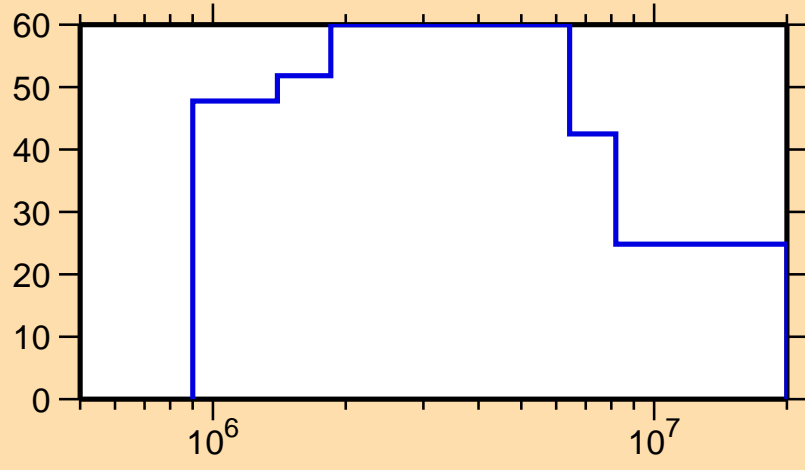
\Delta\sigma/\sigma vs. E for ^{230}\text{Pa}(n,f)
