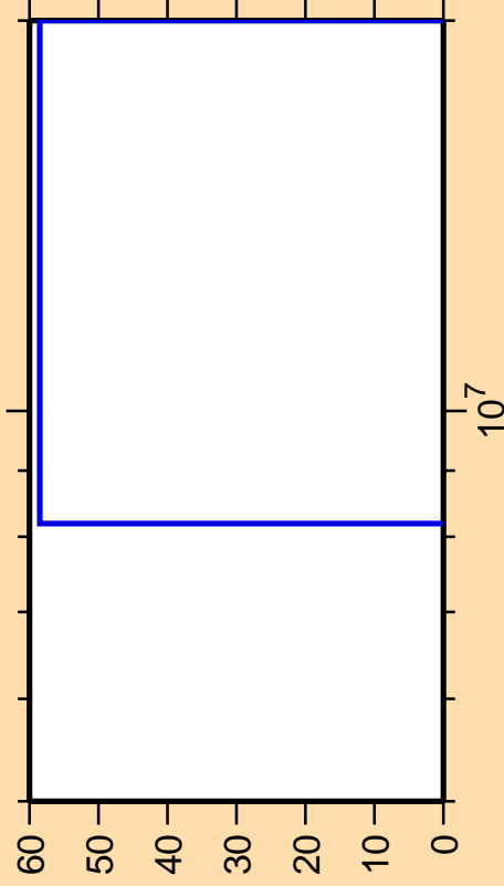
\Delta\sigma/\sigma vs. E for ^{230}\text{Pa}(n,nd)
