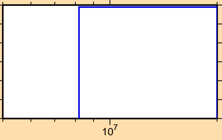
\sigma vs. E for ^{230}\text{Pa} (mt 34)
