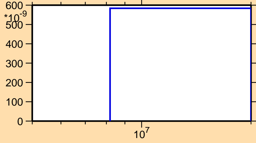
\sigma vs. E for ^{230}\text{Pa}(n,nd)
