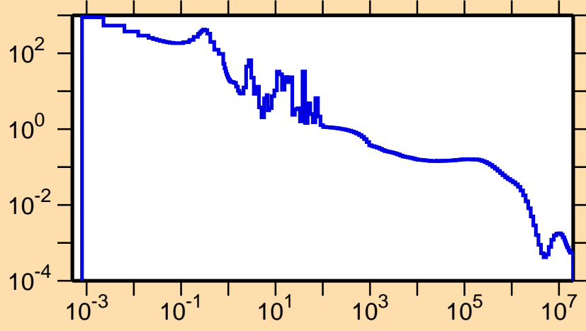
\sigma vs. E for ^{232}\text{Pa}(n,\gamma)
