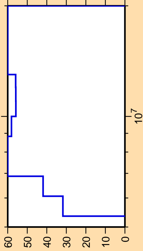
\Delta\sigma/\sigma vs. E for ^{232}\text{Pa}(n,n_1)
