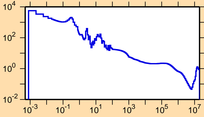
\sigma vs. E for ^{232}\text{Pa}(n,f)
