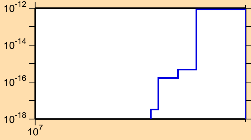
\sigma vs. E for ^{232}\text{Pa} (mt 11)
