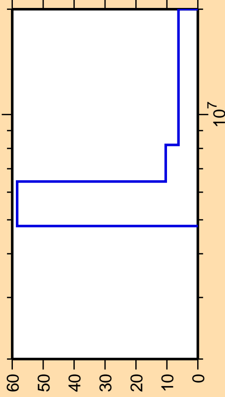
\Delta\sigma/\sigma vs. E for ^{232}\text{Pa}(n,n\text{cont.})
