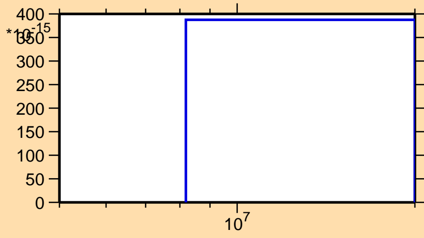
\sigma vs. E for ^{232}\text{Pa}(n,3n\alpha)
