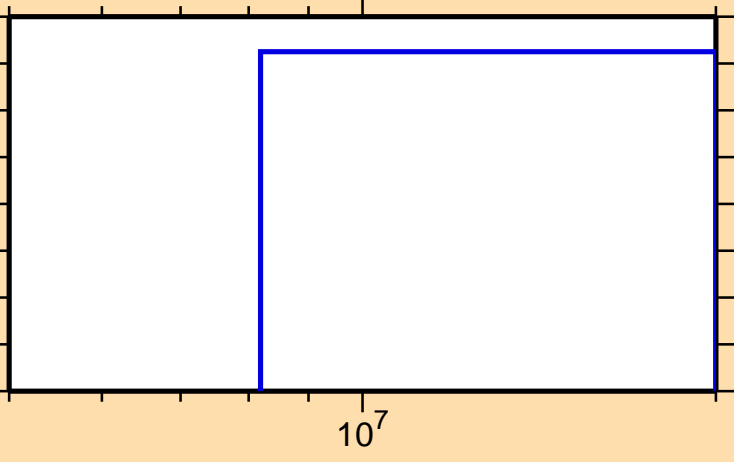
\sigma vs. E for ^{232}\text{Pa}(n,2n\alpha)
