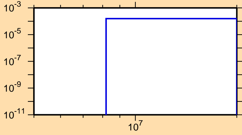
\sigma vs. E for ^{232}\text{Pa}(n,np)
