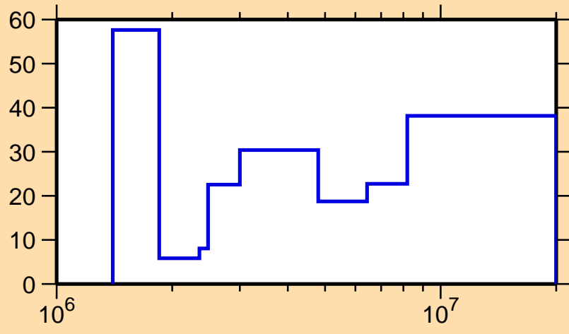
\Delta\sigma/\sigma vs. E for ^{232}\text{Pa}(n,el.)
