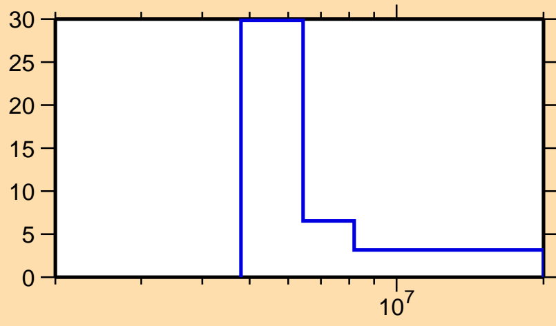
\Delta\sigma/\sigma vs. E for ^{232}\text{Pa}(n,\text{tot.})
