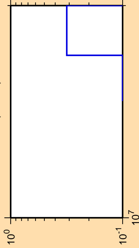
\Delta\sigma/\sigma vs. E for ^{233}\text{Pa} (mt 11)
