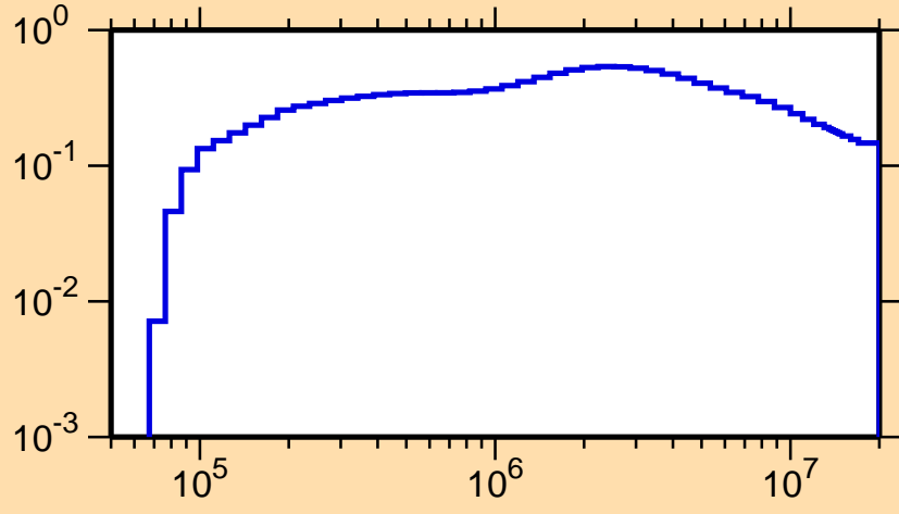
\sigma vs. E for ^{233}\text{Pa}(n,n_3)
