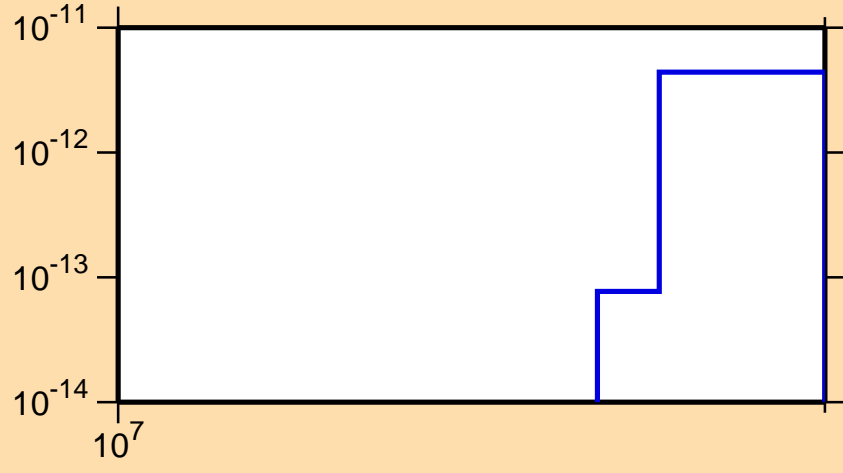
\sigma vs. E for ^{233}\text{Pa}(n,\text{He3})
