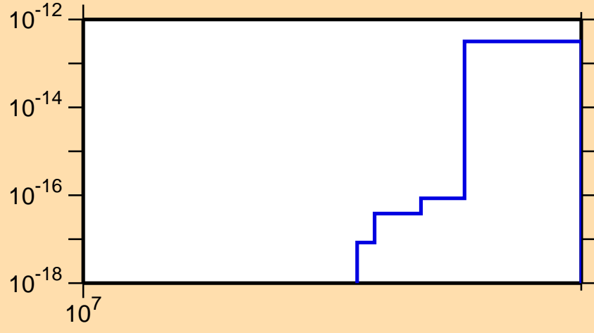
\sigma vs. E for ^{233}\text{Pa} (mt 11)
