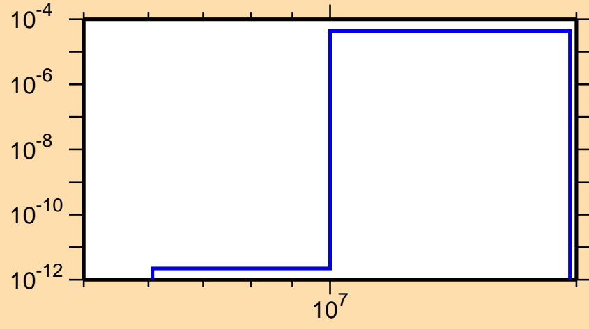
\sigma vs. E for ^{233}\text{Pa}(n,t)
