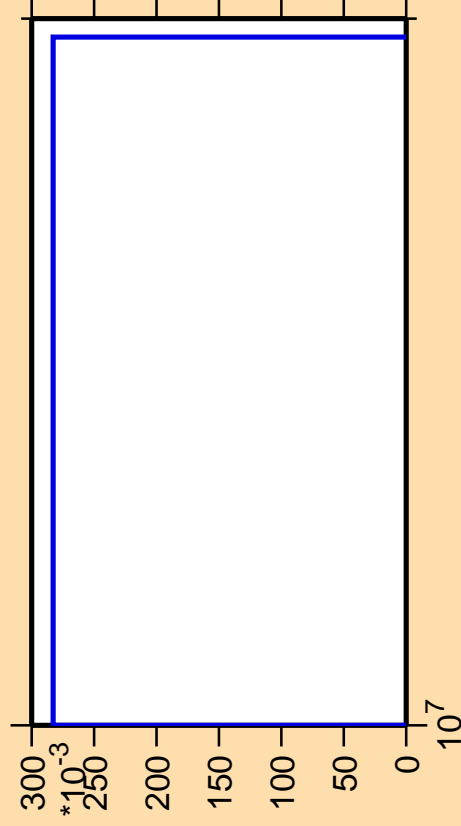
\Delta\sigma/\sigma vs. E for ^{233}\text{Pa}(n,3n\alpha)
