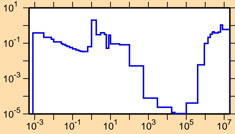
\sigma vs. E for ^{233}\text{Pa}(n,f)
