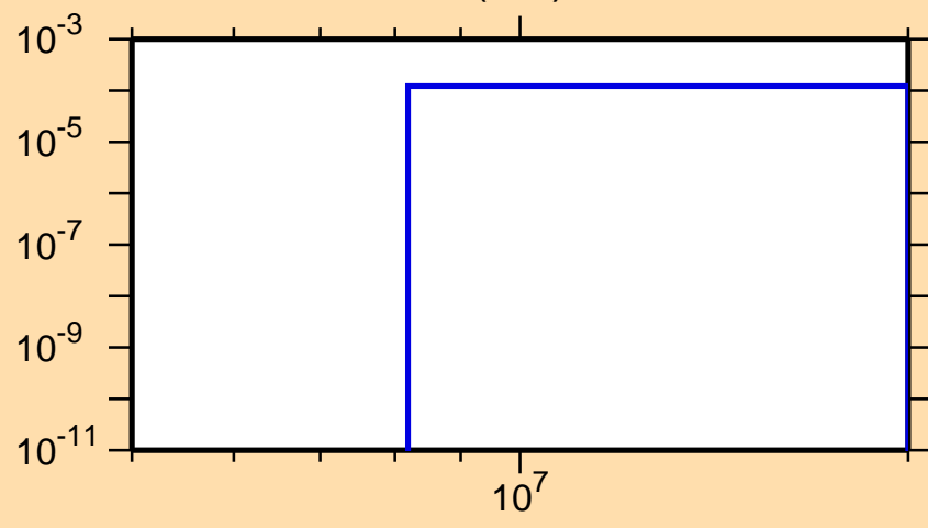
\sigma vs. E for ^{233}\text{Pa}(n,d)
