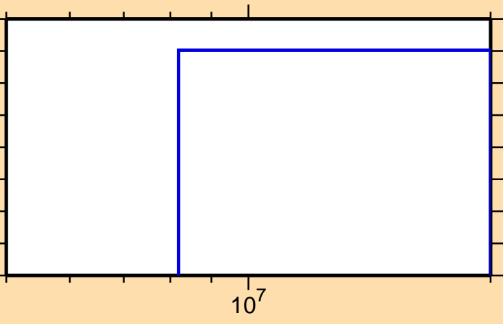
\sigma vs. E for ^{233}\text{Pa}(n,t)
