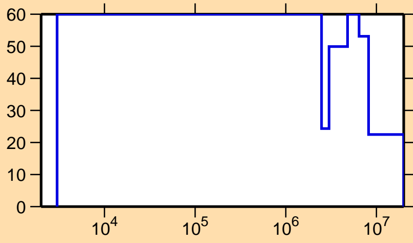
\Delta\sigma/\sigma vs. E for ^{233}\text{Pa}(n,f)
