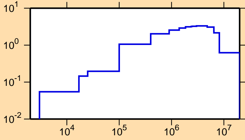
\sigma vs. E for ^{233}\text{Pa}(n,\text{inel.})
