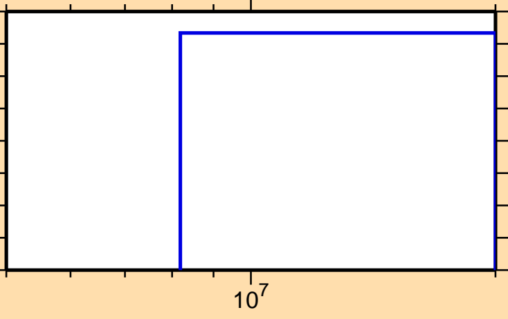
\sigma vs. E for ^{233}\text{Pa}(n,\text{nd})
