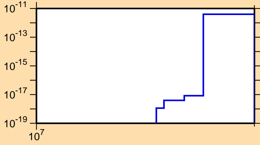
\sigma vs. E for ^{234}\text{Pa} (mt 11)
