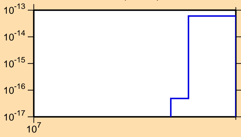
\sigma vs. E for ^{234}\text{Pa} (mt 42)
