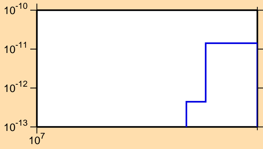
\sigma vs. E for ^{234}\text{Pa}(n,3n\alpha)
