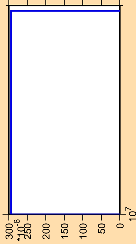
\Delta\sigma/\sigma vs. E for ^{234}\text{Pa} (mt 42)
