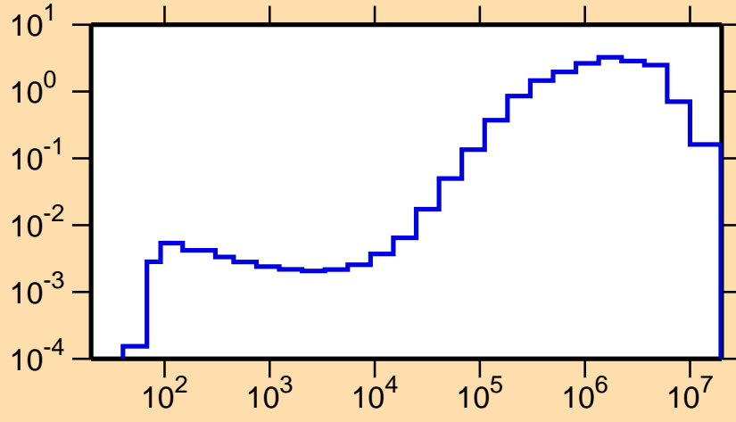
\sigma vs. E for ^{234}\text{Pa}(n,\text{inel.})
