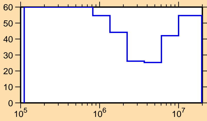
\Delta\sigma/\sigma vs. E for ^{234}\text{Pa}(n,n\text{cont.})
