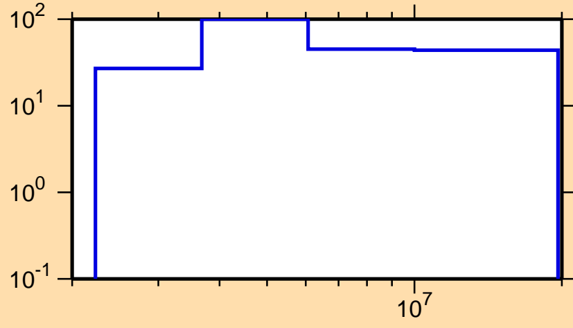
\Delta\sigma/\sigma vs. E for ^{234}\text{Pa}(n,p)
