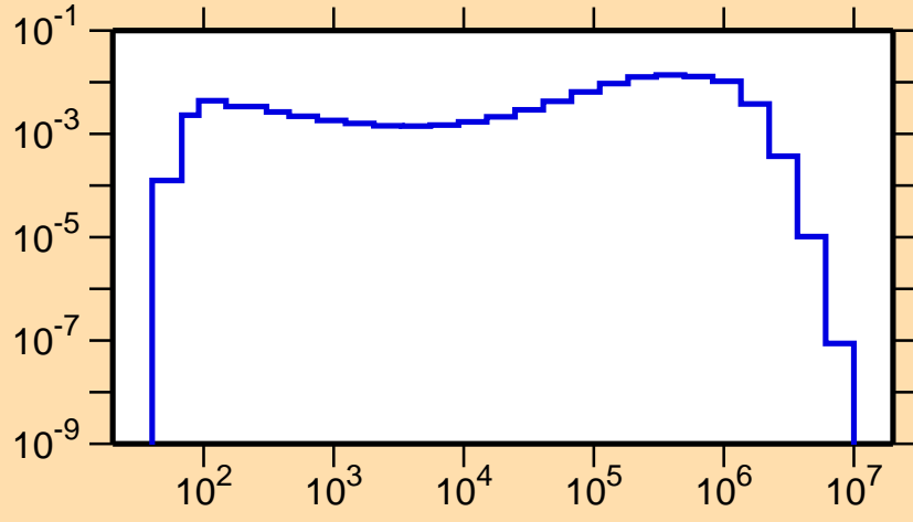
\sigma vs. E for ^{234}\text{Pa}(n,n_1)
