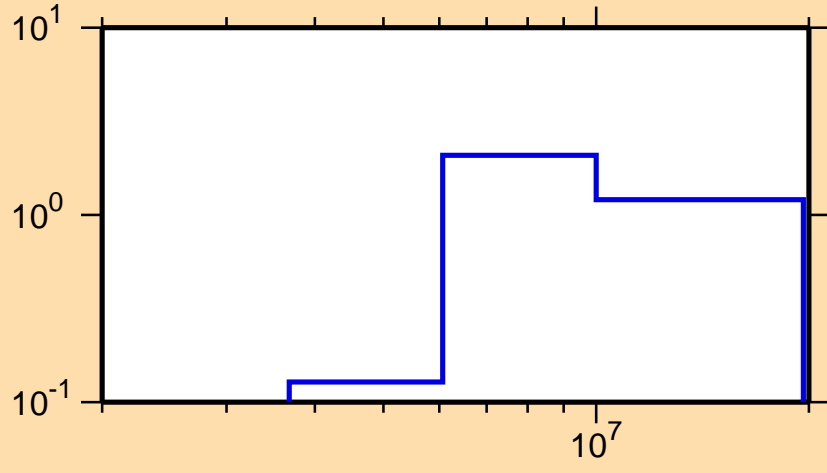
\sigma vs. E for ^{234}\text{Pa}(n,2n)
