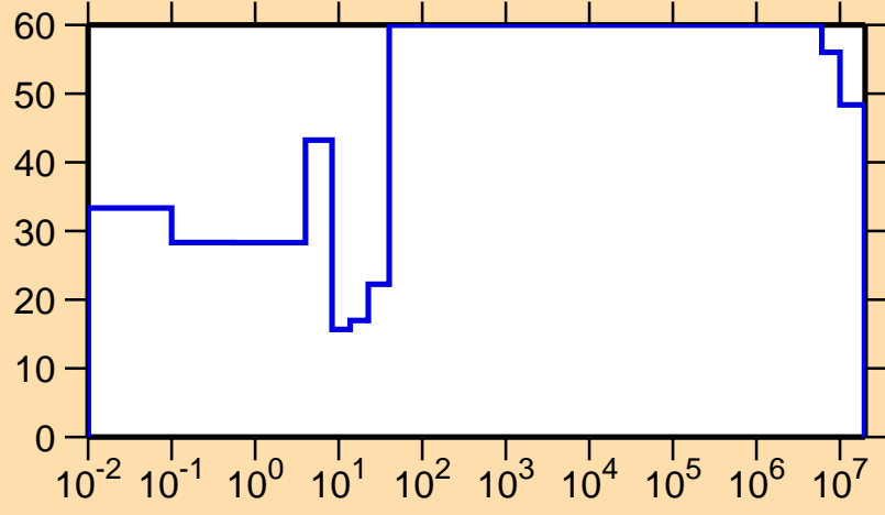
\Delta\sigma/\sigma vs. E for ^{234}\text{Pa}(n,\gamma)
