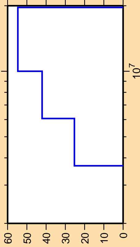
\Delta\sigma/\sigma vs. E for ^{234}\text{Pa}(n,n\text{cont.})
