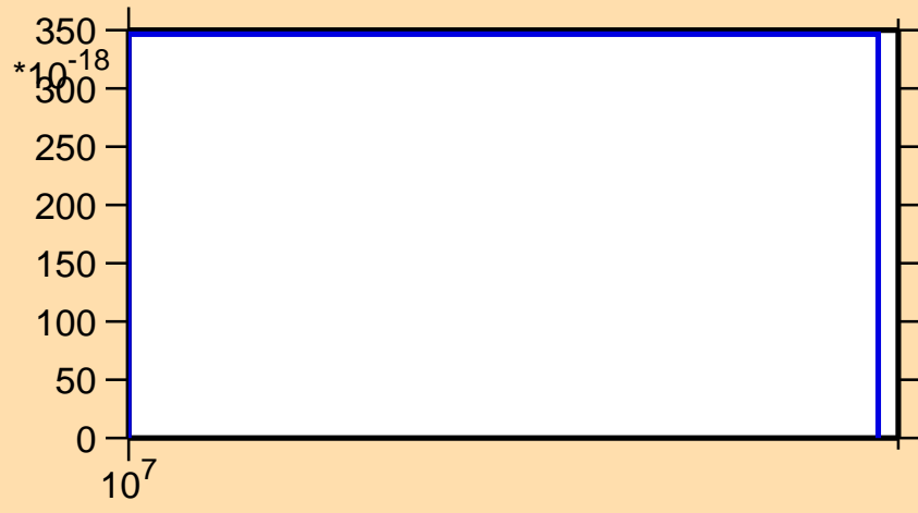
\sigma vs. E for ^{234}\text{Pa} (mt 42)
