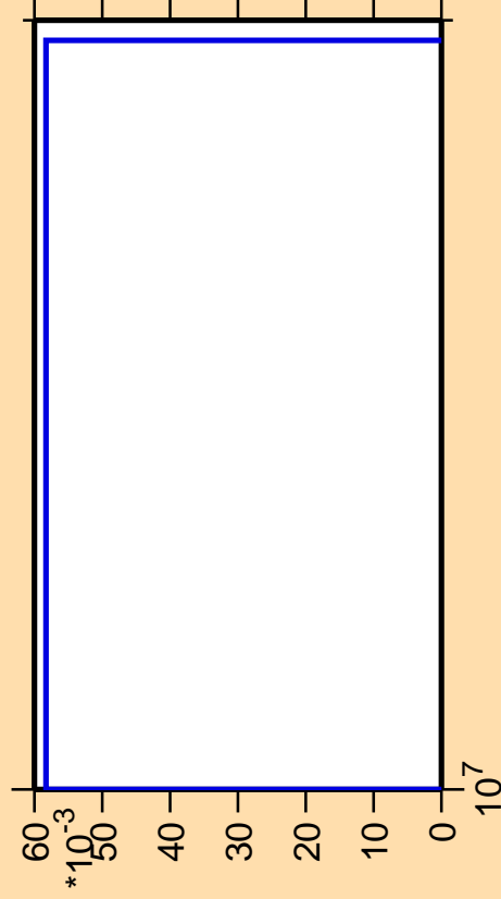
\Delta\sigma/\sigma vs. E for ^{234}\text{Pa}(n,\text{He}3)
