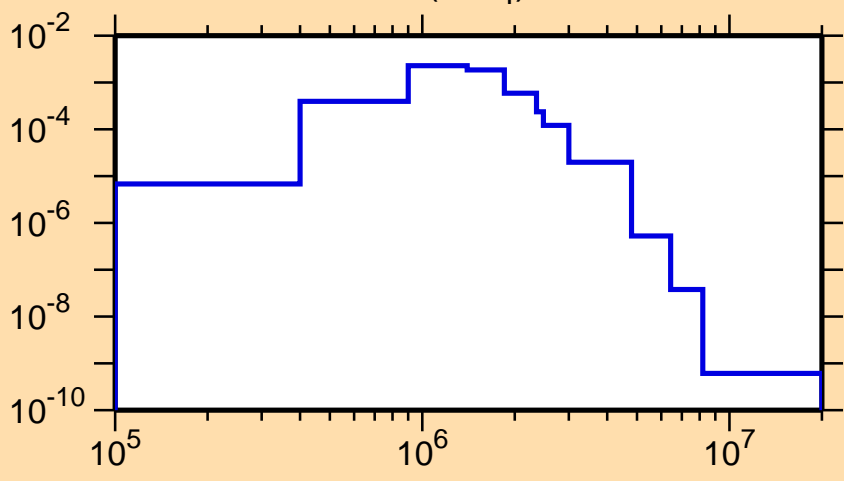
\sigma vs. E for ^{234}\text{Pa}(n,n_4)
