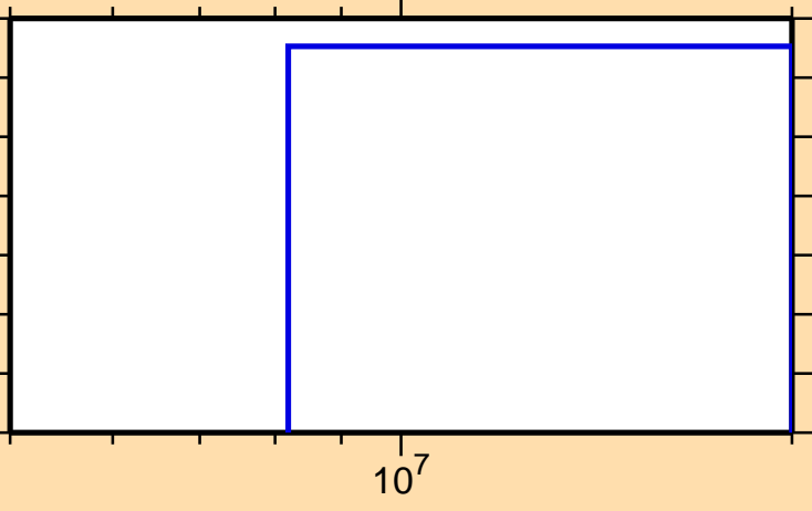
\sigma vs. E for ^{234}\text{Pa}(n,2n\alpha)
