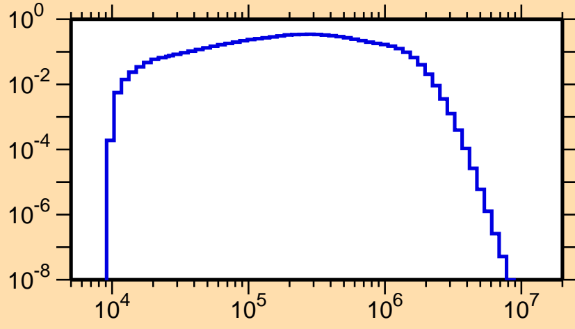
\sigma vs. E for ^{235}\text{Pa}(n,n_1)
