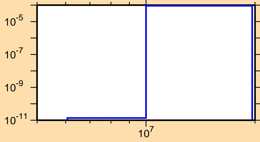
\sigma vs. E for ^{235}\text{Pa}(n,np)
