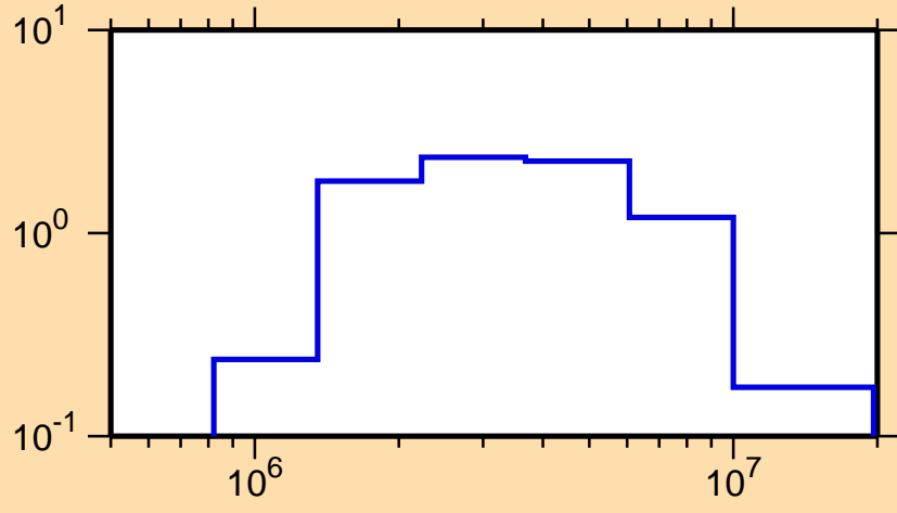
\sigma vs. E for ^{235}\text{Pa}(n,n\text{cont.})
