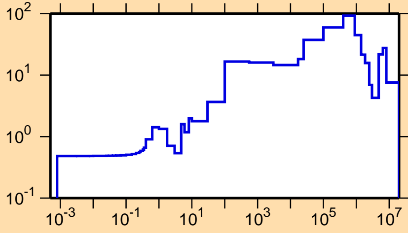
\Delta\sigma/\sigma vs. E for ^{235}\text{Pa}(n,el.)
