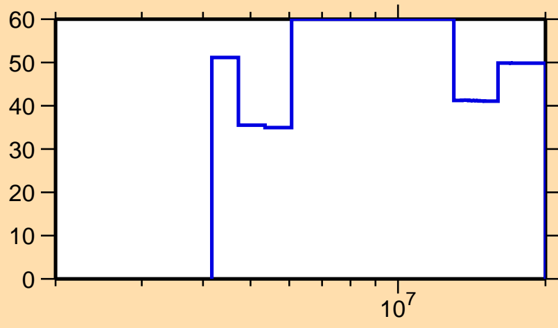
\Delta\sigma/\sigma vs. E for ^{238}\text{Pa}(n,p)
