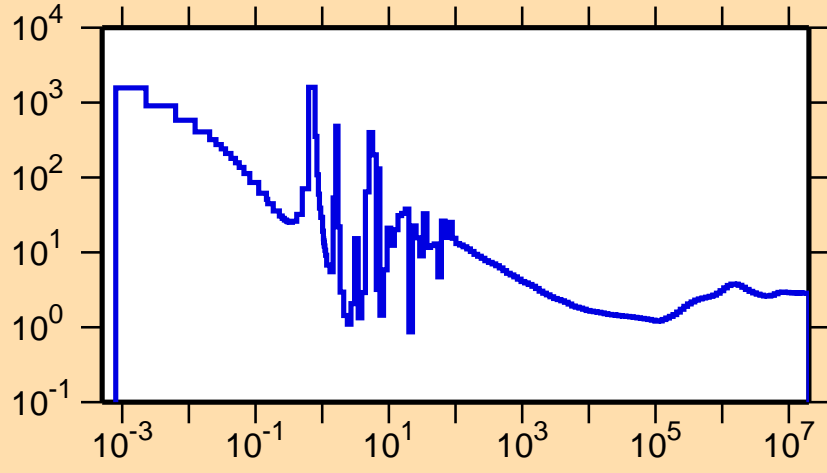
\sigma vs. E for ^{238}\text{Pa}(n,\text{nonel.})
