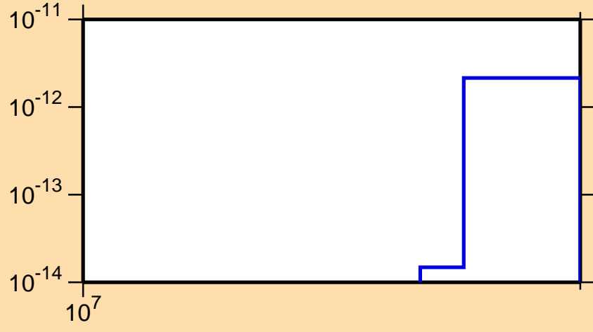
\sigma vs. E for ^{238}\text{Pa}(n,3n\alpha)
