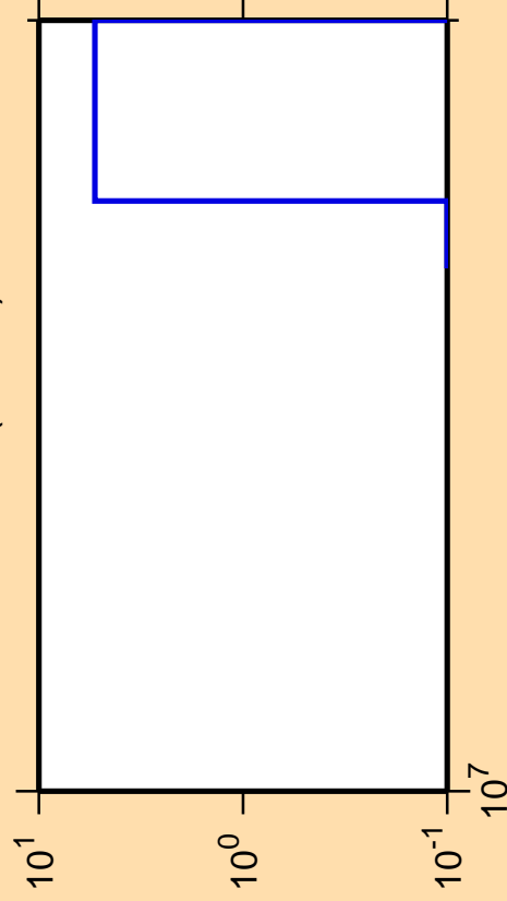
\Delta\sigma/\sigma vs. E for ^{238}\text{Pa} (mt 11)
