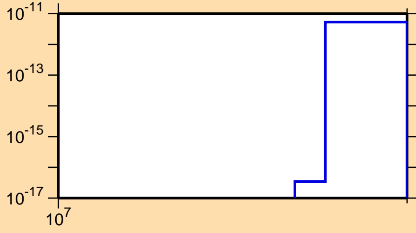
\sigma vs. E for ^{238}\text{Pa} (mt 11)
