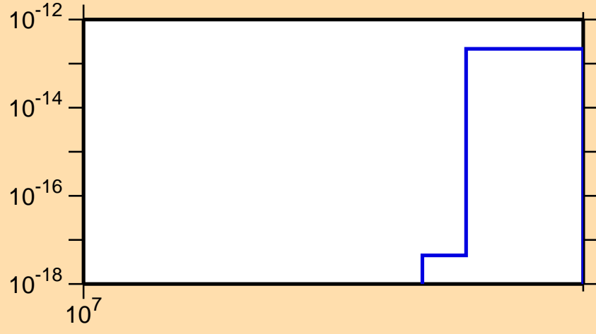
\sigma vs. E for ^{238}\text{Pa} (mt 42)
