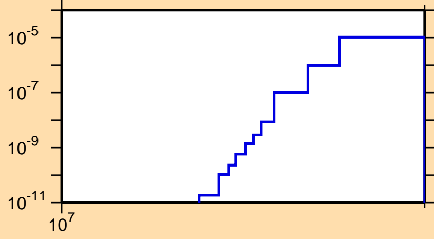
\sigma vs. E for ^{238}\text{Pa}(n,\text{nd})
