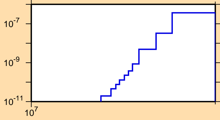
\sigma vs. E for ^{238}\text{Pa}(n,2n\alpha)
