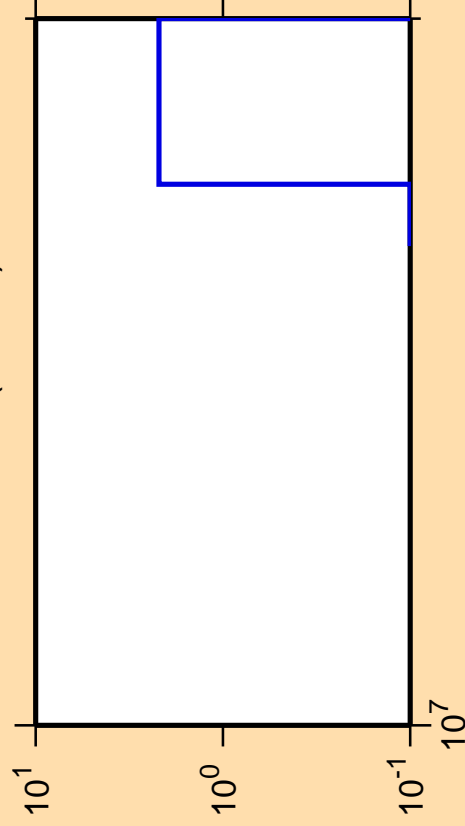
\Delta\sigma/\sigma vs. E for ^{238}\text{Pa}(n,\text{He3})
