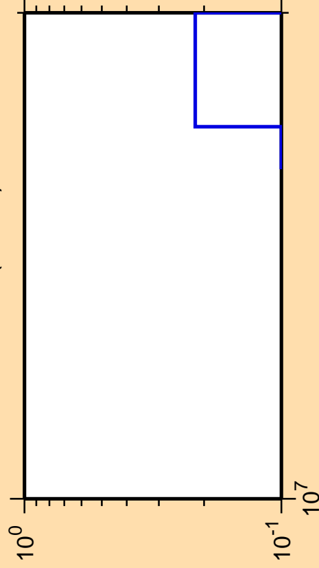
\Delta\sigma/\sigma vs. E for ^{238}\text{Pa} (mt 42)
