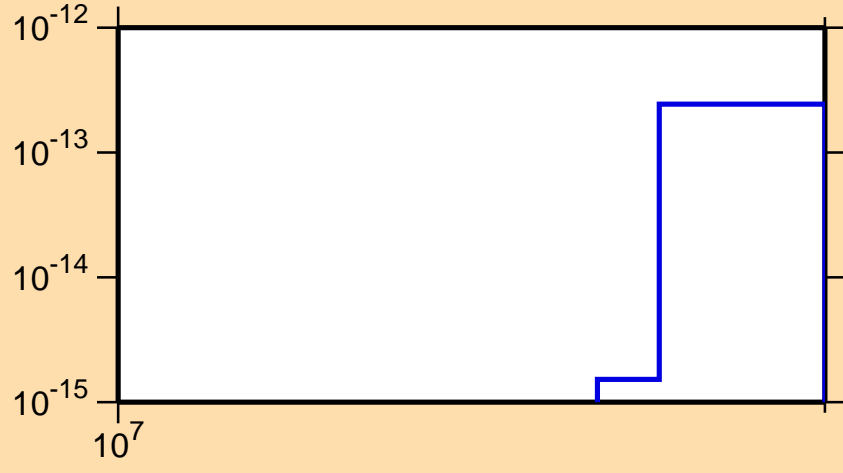
\sigma vs. E for ^{238}\text{Pa}(n,\text{He3})
