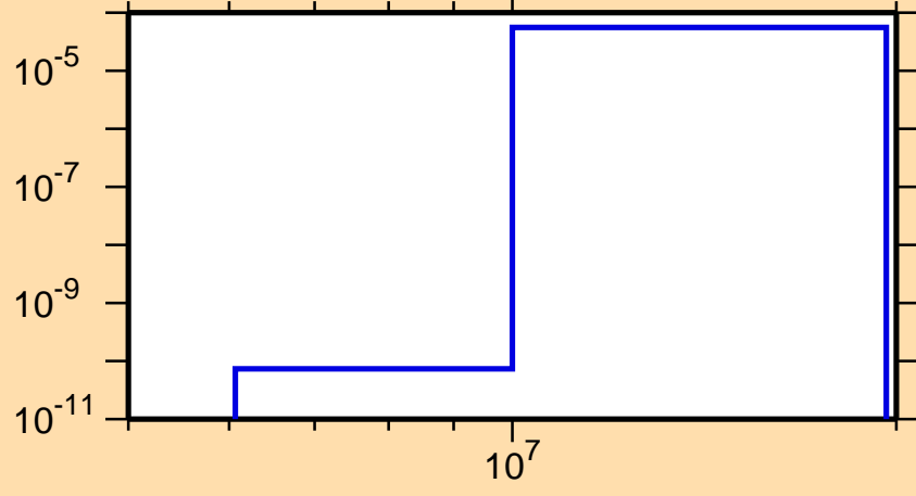
\sigma vs. E for ^{238}\text{Pa}(n,t)
