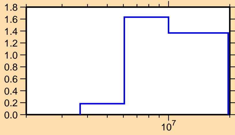
\sigma vs. E for ^{238}\text{Pa}(n,2n)
