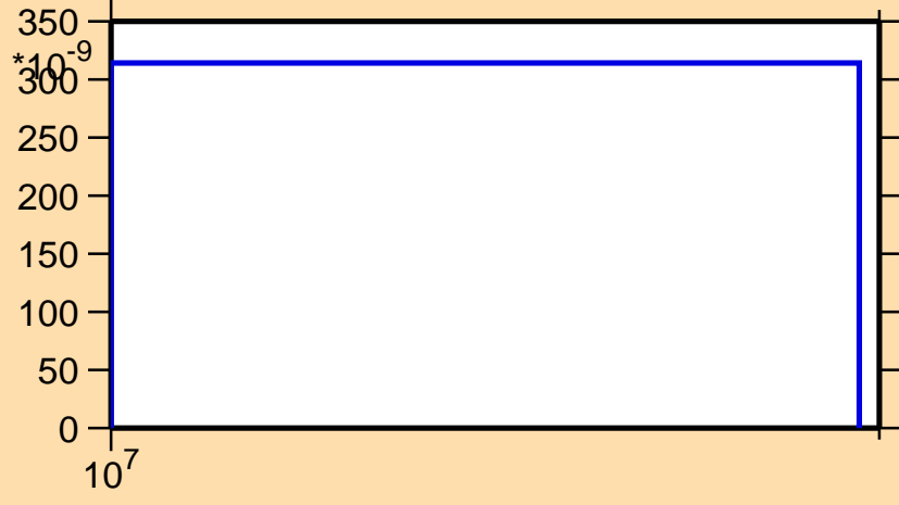
\sigma vs. E for ^{238}\text{Pa}(n,nt)
