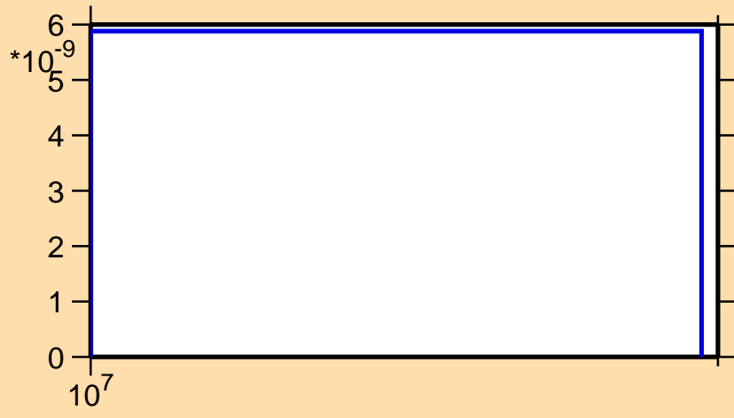
\sigma vs. E for ^{238}\text{Pa}(n,2n\alpha)
