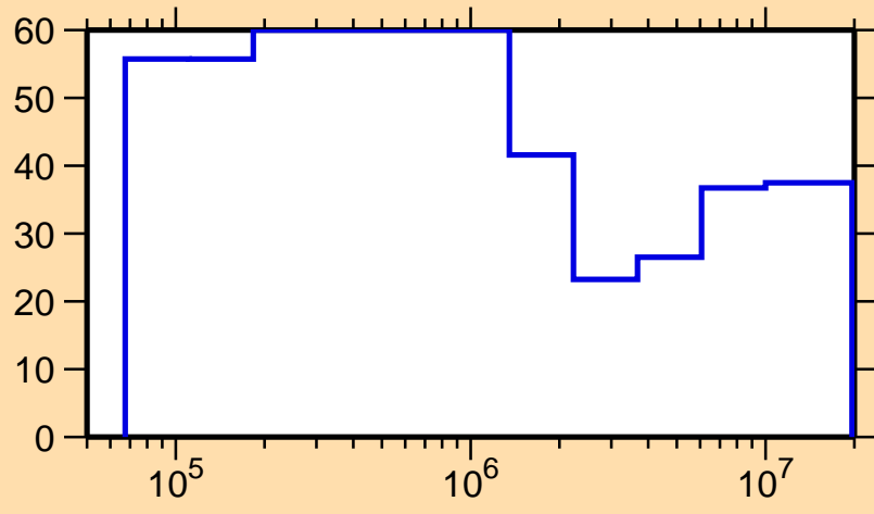
\Delta\sigma/\sigma vs. E for ^{238}\text{Pa}(n,\text{el.})
