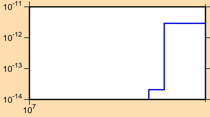
\sigma vs. E for ^{239}\text{Pa}(n,3n\alpha)
