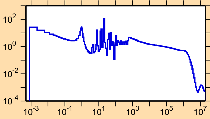
\sigma vs. E for ^{239}\text{Pa}(n,\gamma)
