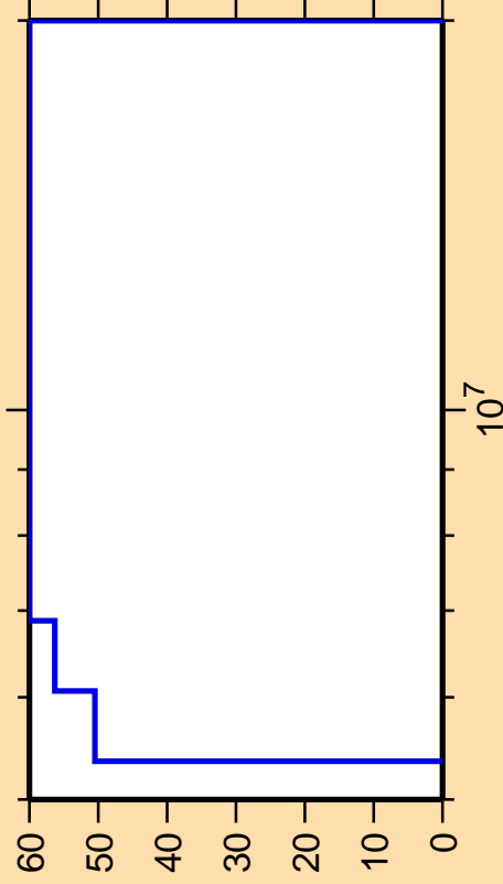
\Delta\sigma/\sigma vs. E for ^{239}\text{Pa}(n,n\text{cont.})
