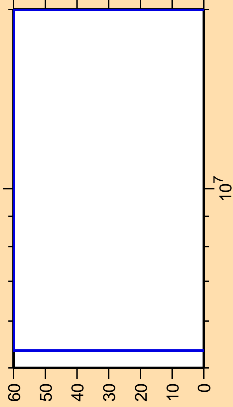
\Delta\sigma/\sigma vs. E for ^{239}\text{Pa}(n,f)
