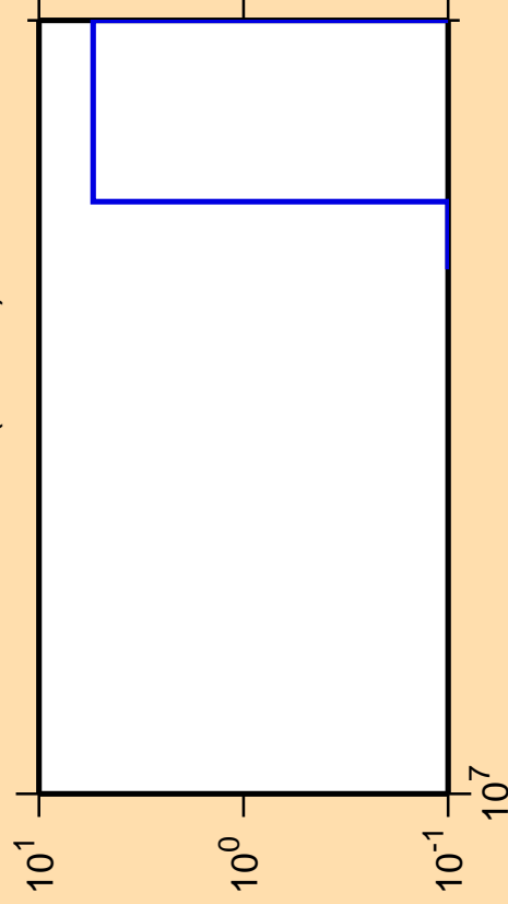
\Delta\sigma/\sigma vs. E for ^{239}\text{Pa} (mt 11)
