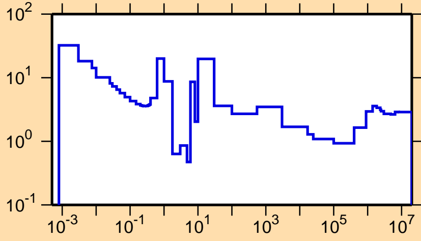
\sigma vs. E for ^{239}\text{Pa}(n,\text{nonel.})
