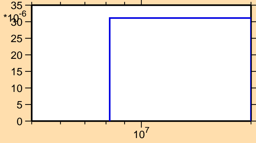
\sigma vs. E for ^{239}\text{Pa}(n,d)
