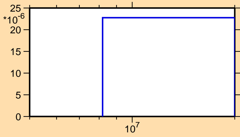
\sigma vs. E for ^{239}\text{Pa}(n,np)
