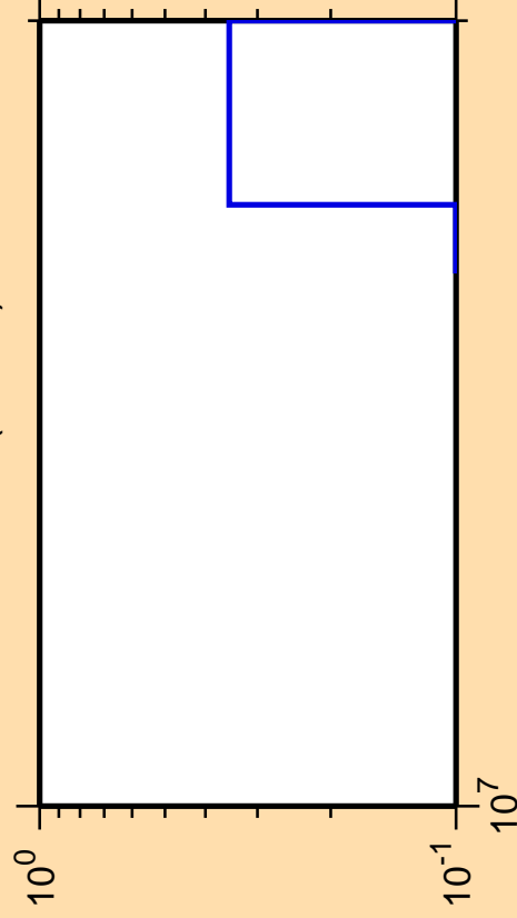
\Delta\sigma/\sigma vs. E for ^{240}\text{Pa} (mt 42)
