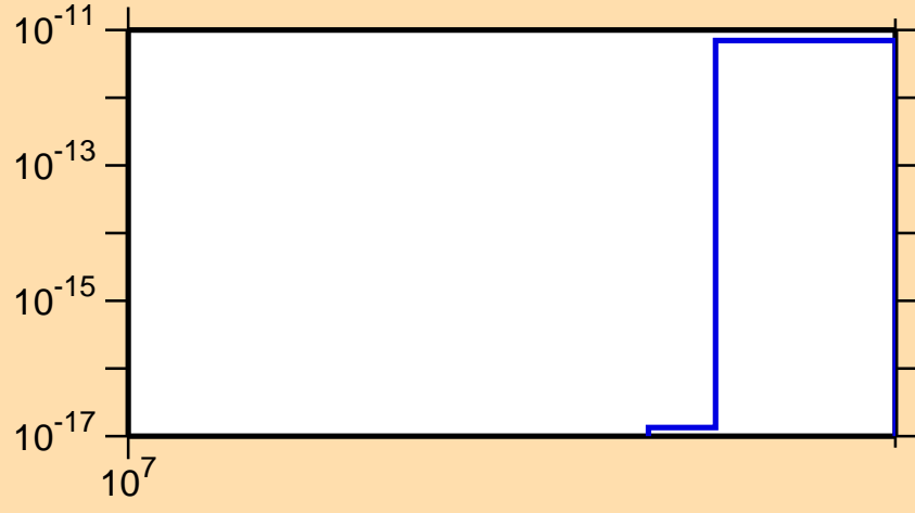
\sigma vs. E for ^{240}\text{Pa} (mt 11)
