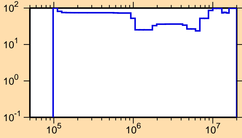
\Delta\sigma/\sigma vs. E for ^{240}\text{Pa}(n,n\text{cont.})
