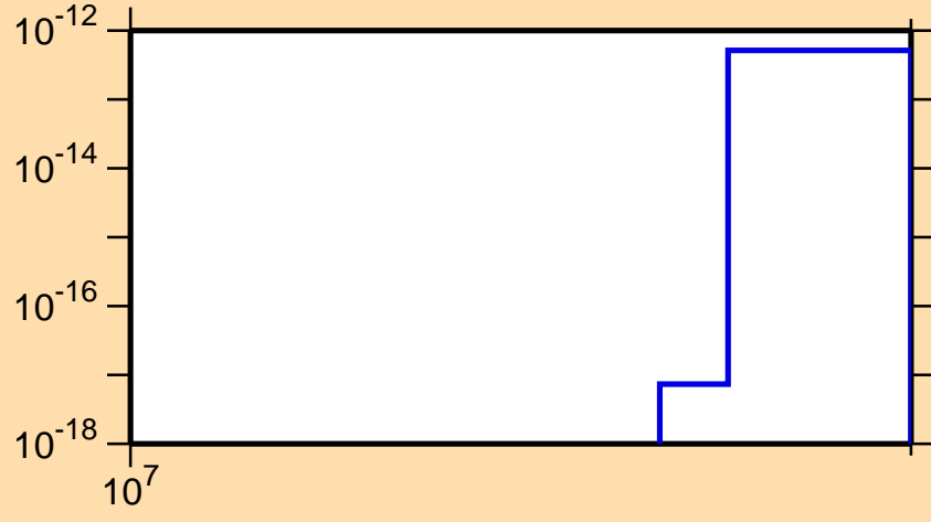
\sigma vs. E for ^{240}\text{Pa} (mt 42)
