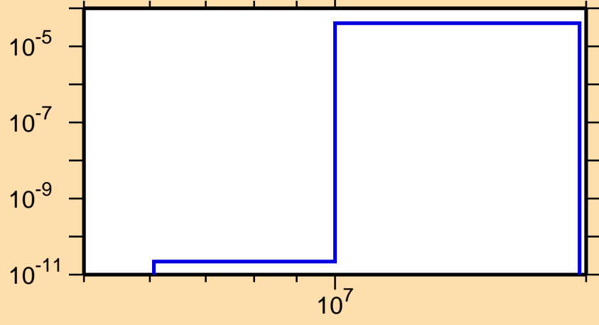
\sigma vs. E for ^{240}\text{Pa}(n,t)
