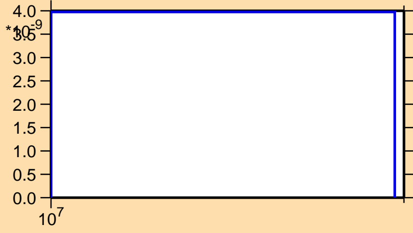
\sigma vs. E for ^{240}\text{Pa}(n,2n\alpha)
