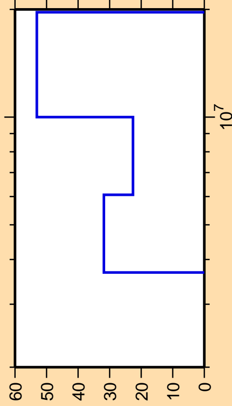
\Delta\sigma/\sigma vs. E for ^{240}\text{Pa}(n,2n)
