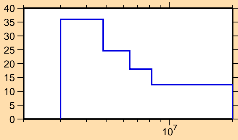
\Delta\sigma/\sigma vs. E for ^{240}\text{Pa}(n,\text{nonel.})
