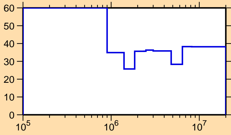
\Delta\sigma/\sigma vs. E for ^{240}\text{Pa}(n,\text{inel.})
