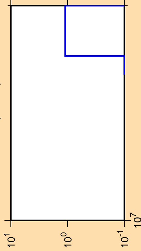
\Delta\sigma/\sigma vs. E for ^{241}\text{Pa} (mt 42)
