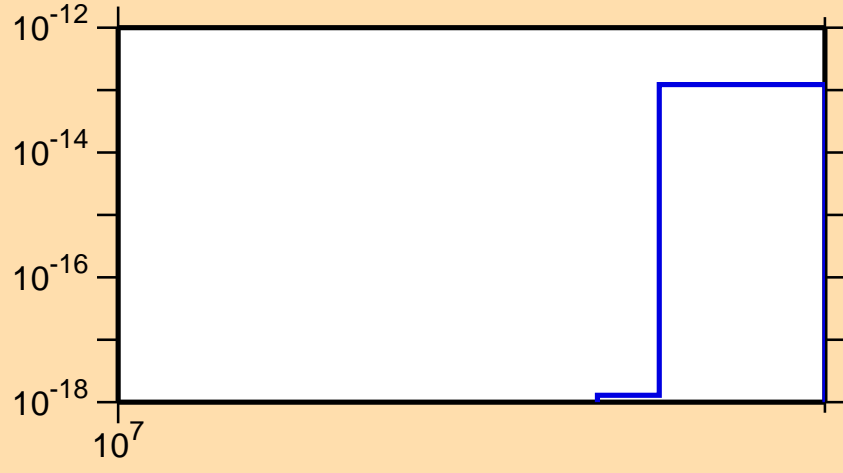
\sigma vs. E for ^{241}\text{Pa} (mt 42)
