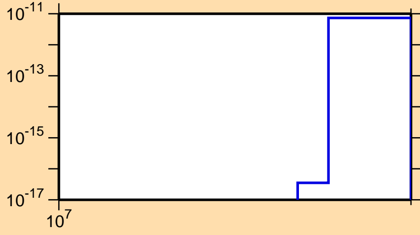
\sigma vs. E for ^{241}\text{Pa} (mt 11)
