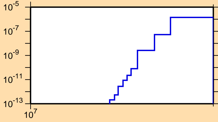
\sigma vs. E for ^{241}\text{Pa}(n,\text{nd})
