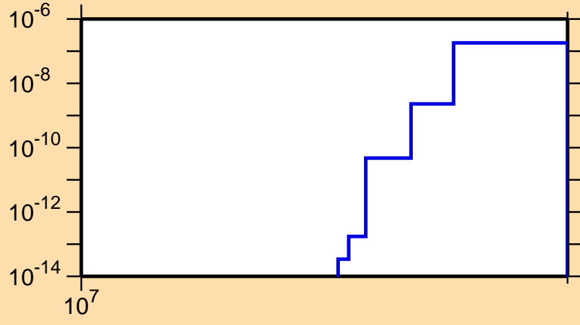
\sigma vs. E for ^{241}\text{Pa}(n,2np)
