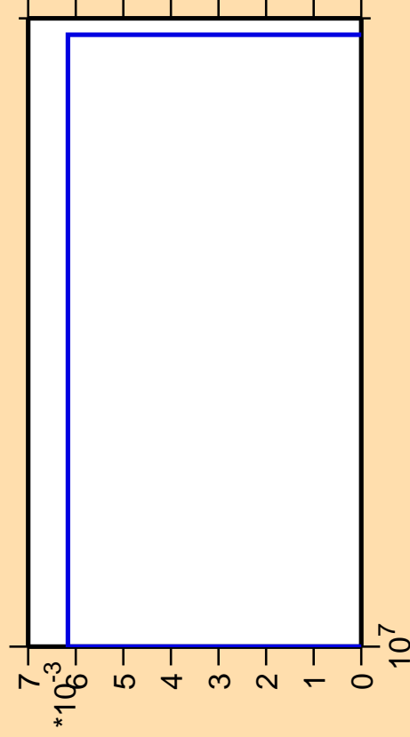
\Delta\sigma/\sigma vs. E for ^{241}\text{Pa} (mt 42)
