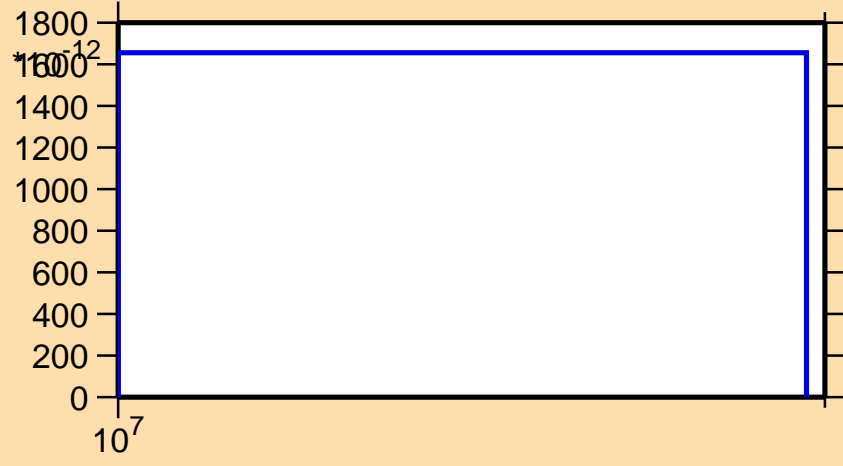
\sigma vs. E for ^{241}\text{Pa}(n,2np)
