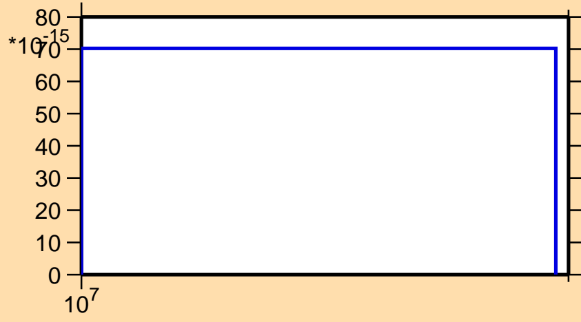
\sigma vs. E for ^{241}\text{Pa}(n,3n\alpha)
