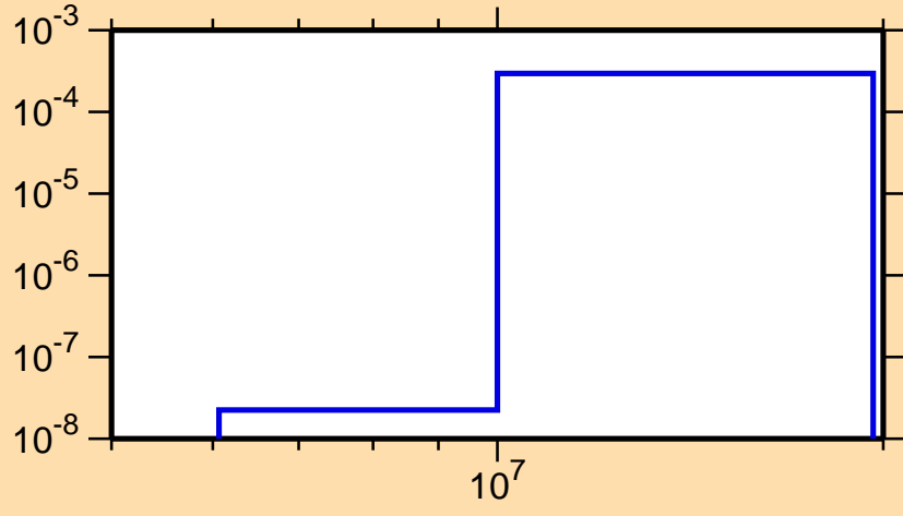
\sigma vs. E for ^{241}\text{Pa}(n,p)
