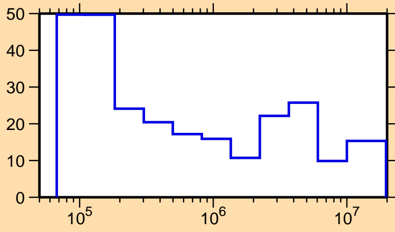
\Delta\sigma/\sigma vs. E for ^{241}\text{Pa}(n,\text{tot.})
