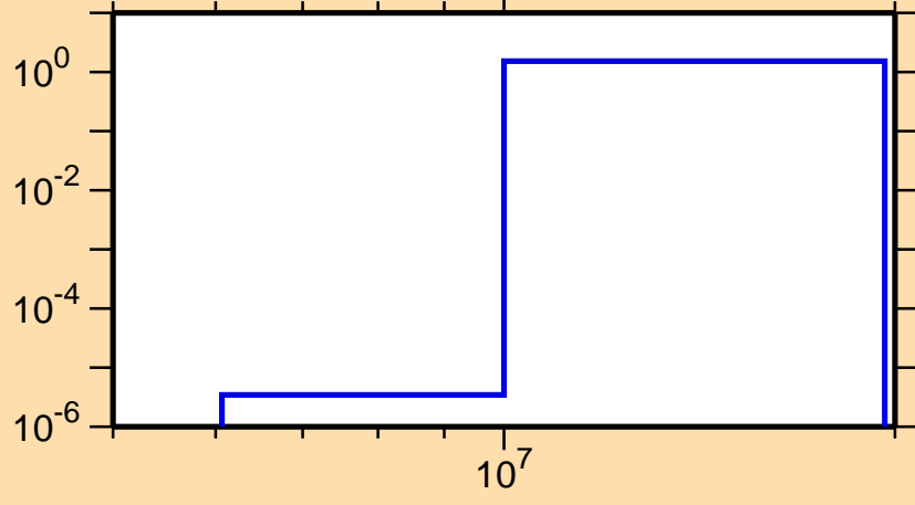
\sigma vs. E for ^{241}\text{Pa}(n,3n)
