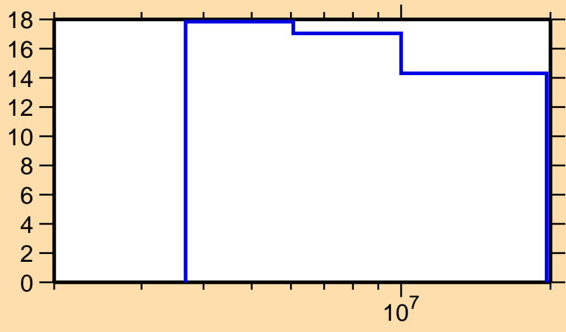
\Delta\sigma/\sigma vs. E for ^{241}\text{Pa}(n,\text{nonel.})
