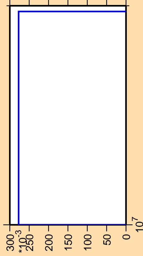
\Delta\sigma/\sigma vs. E for ^{241}\text{Pa} (mt 11)
