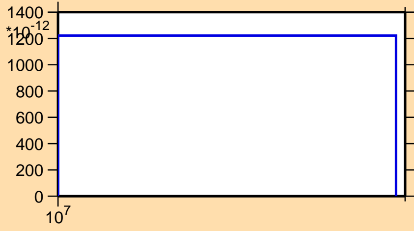
\sigma vs. E for ^{241}\text{Pa}(n,2n\alpha)
