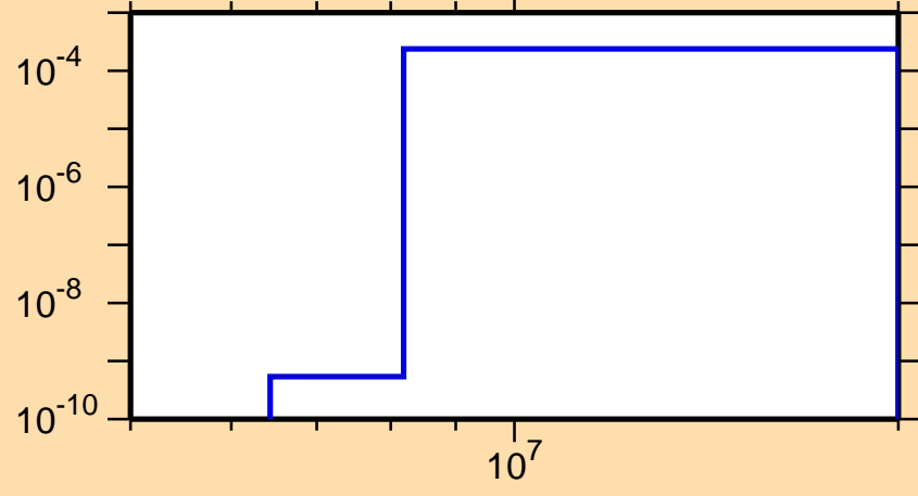
\sigma vs. E for ^{241}\text{Pa}(n,p)
