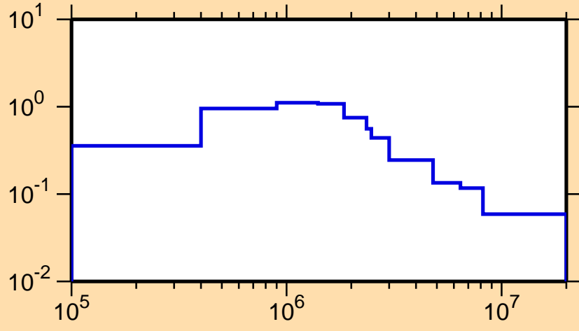
\sigma vs. E for ^{241}\text{Pa}(n,n_1)
