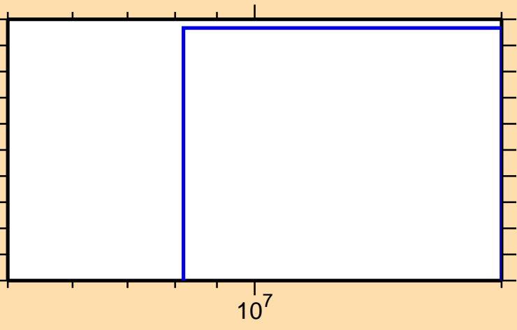
\sigma vs. E for ^{241}\text{Pa}(n,t)
