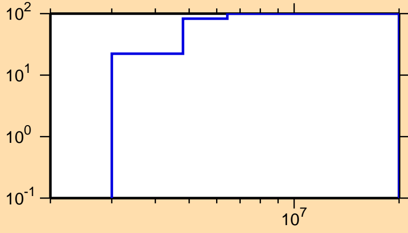
\Delta\sigma/\sigma vs. E for ^{241}\text{Pa}(n,n\text{cont.})
