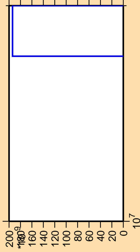
\Delta\sigma/\sigma vs. E for ^{185}\text{Pb} (mt 11)
