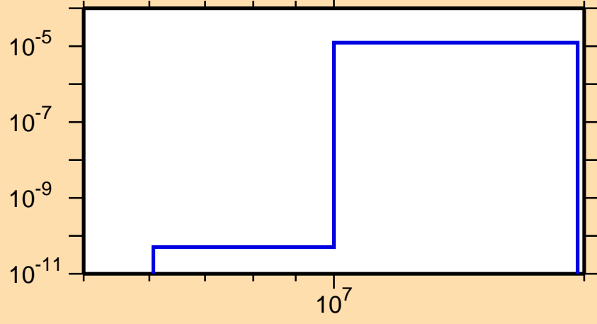
\sigma vs. E for ^{185}\text{Pb}(n,\text{pd})
