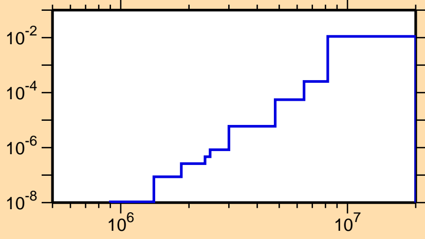
\sigma vs. E for ^{185}\text{Pb}(n,n\alpha)
