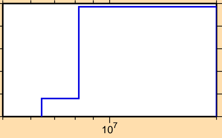
\sigma vs. E for ^{185}\text{Pb}(\text{mt117})
