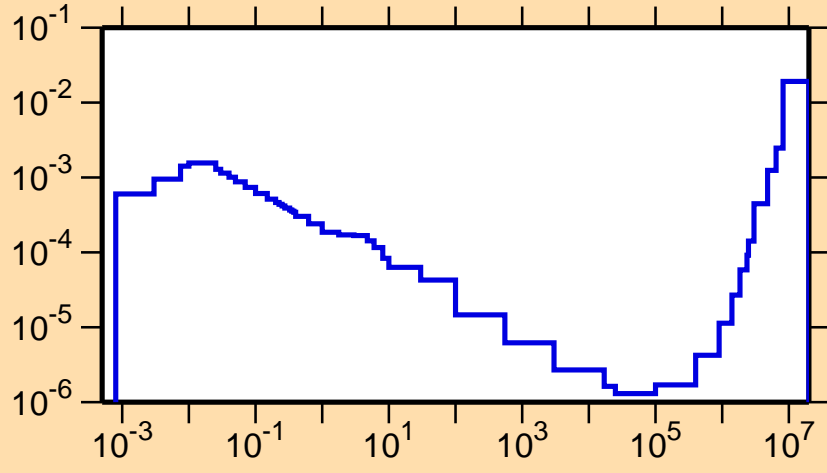
\sigma vs. E for ^{185}\text{Pb}(n,p\alpha)
