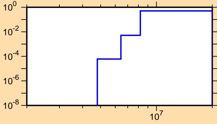
\sigma vs. E for ^{185}\text{Pb}(n,np)
