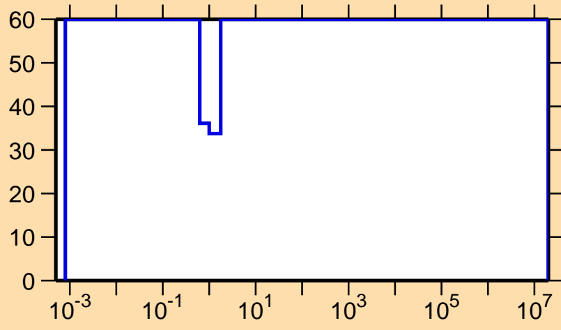
\Delta\sigma/\sigma vs. E for ^{185}\text{Pb}(n,\gamma)
