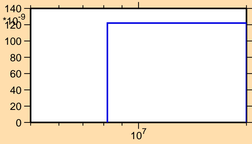
\sigma vs. E for ^{185}\text{Pb}(n,\text{nd})
