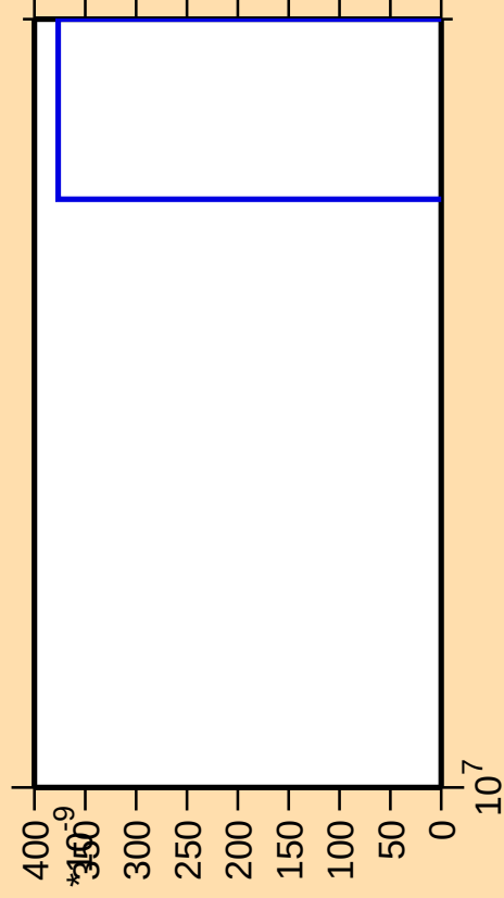
\Delta\sigma/\sigma vs. E for ^{185}\text{Pb}(\text{mt 11})
