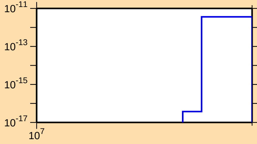
\sigma vs. E for ^{185}\text{Pb}(n,nt)
