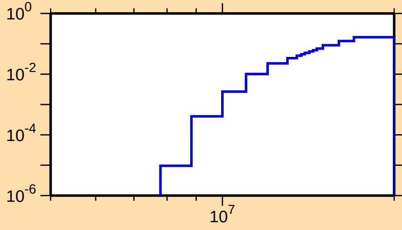
\sigma vs. E for ^{185}\text{Pb}(n,2n)
