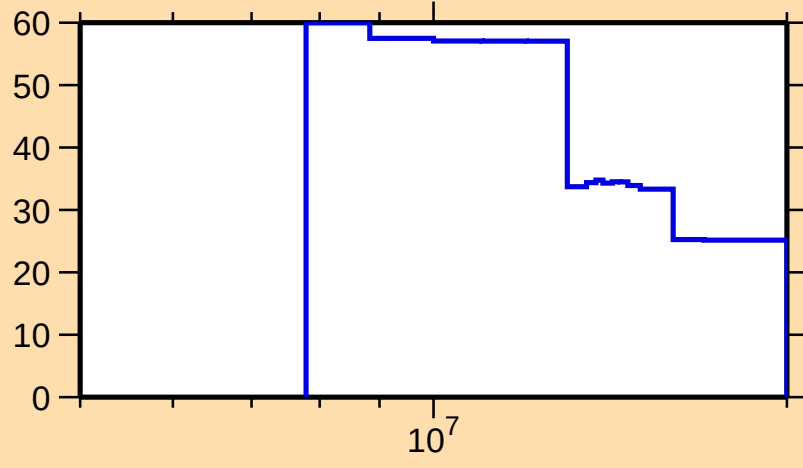
\Delta\sigma/\sigma vs. E for ^{185}\text{Pb}(n,\text{tot.})
