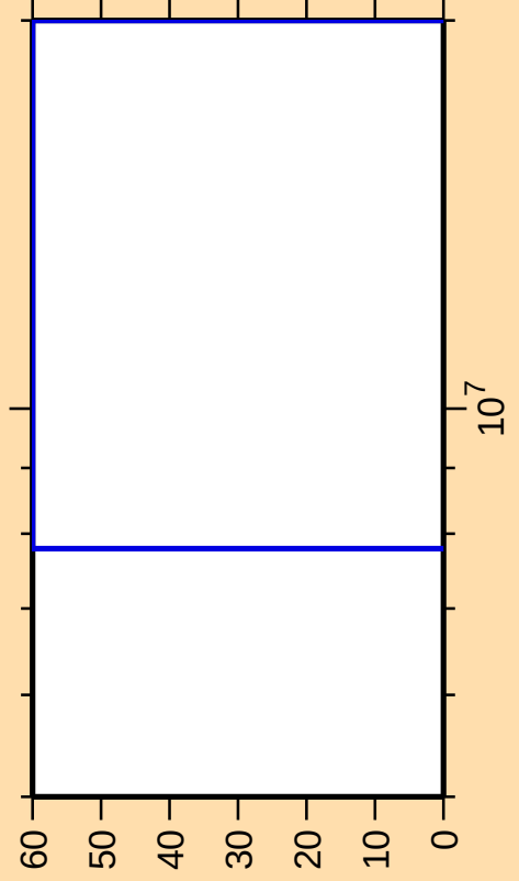
\Delta\sigma/\sigma vs. E for ^{185}\text{Pb}(n,p)
