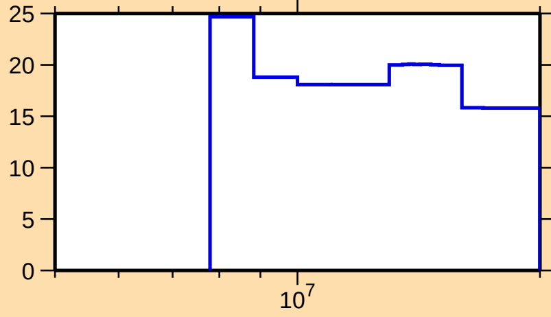
\Delta\sigma/\sigma vs. E for ^{185}\text{Pb}(n,\text{nonel.})
