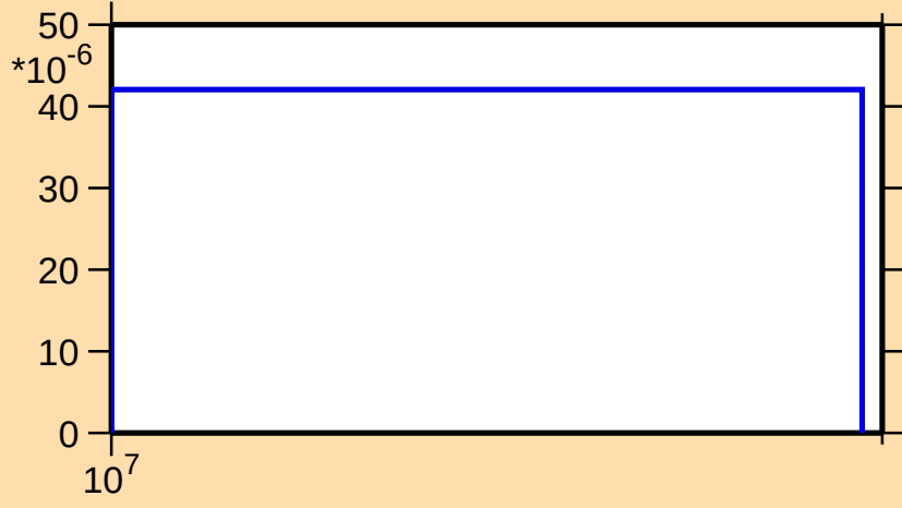
\sigma vs. E for ^{185}\text{Pb}(n,2np)
