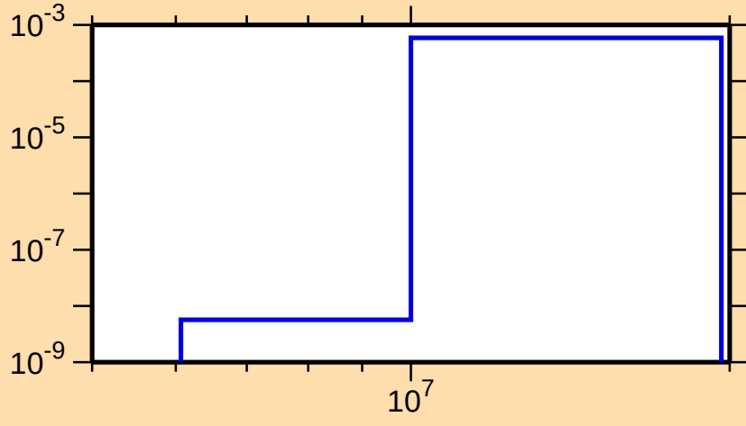
\sigma vs. E for ^{185}\text{Pb}(n,t)
