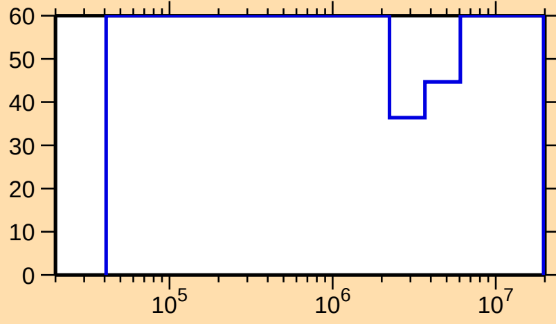
\Delta\sigma/\sigma vs. E for ^{185}\text{Pb}(n,\text{el.})
