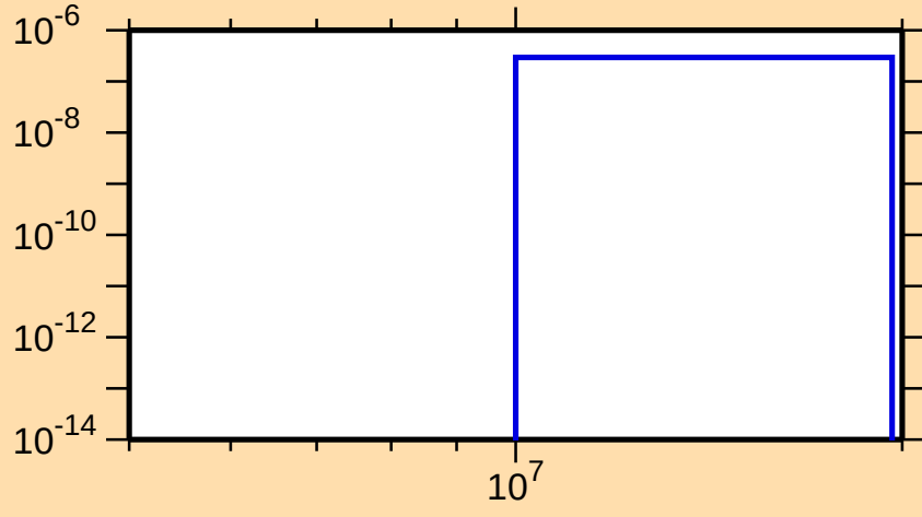
\sigma vs. E for ^{185}\text{Pb}(n,\text{pt})
