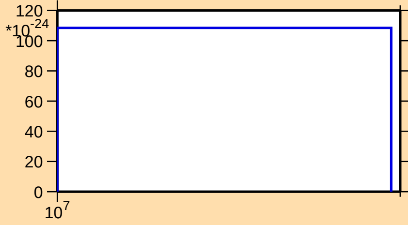
\sigma vs. E for ^{185}\text{Pb}(\text{mt 11})
