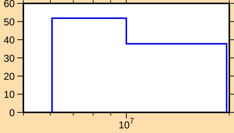
\Delta\sigma/\sigma vs. E for ^{185}\text{Pb}(n,\text{tot.})
