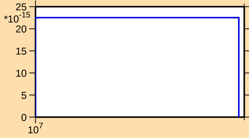
\sigma vs. E for ^{185}\text{Pb}(n,nt)
