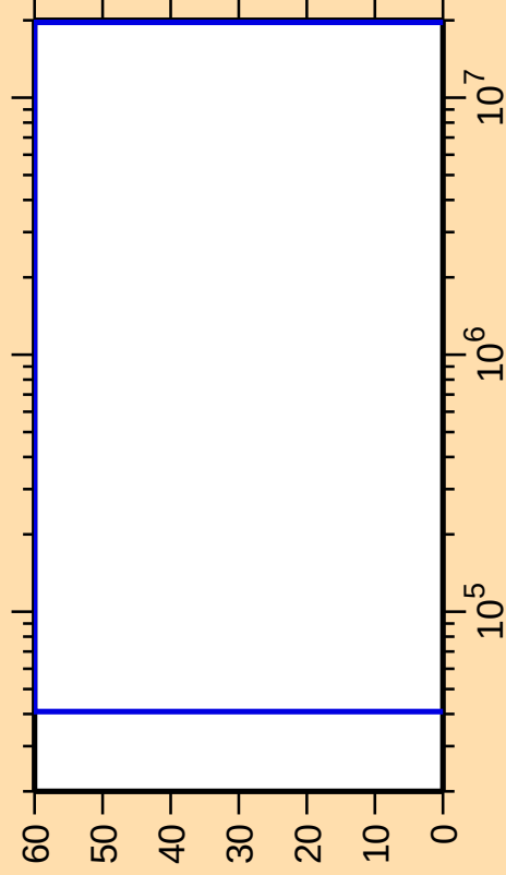
\Delta\sigma/\sigma vs. E for ^{185}\text{Pb}(n,\text{ncont.})
