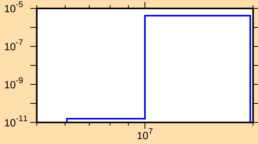
\sigma vs. E for ^{185}\text{Pb}(n,\text{pd})
