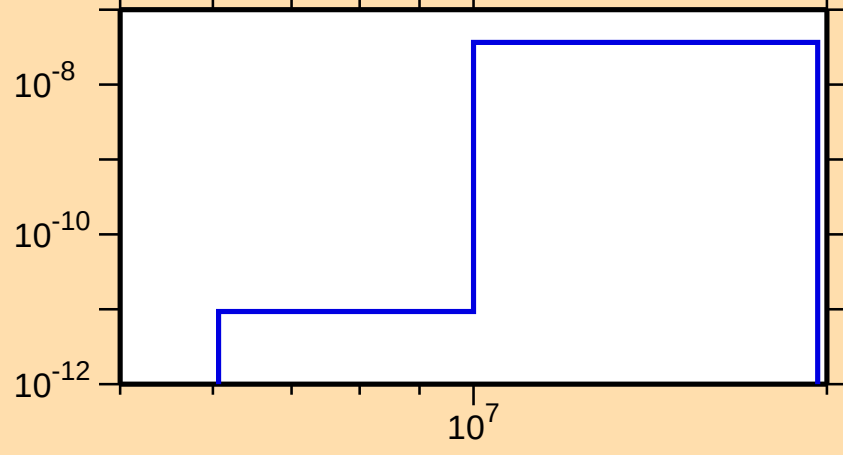
\sigma vs. E for ^{185}\text{Pb}(\text{mt117})
