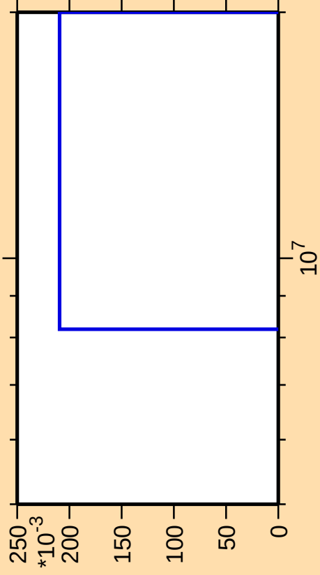
\Delta\sigma/\sigma vs. E for ^{185}\text{Pb}(n,nt)
