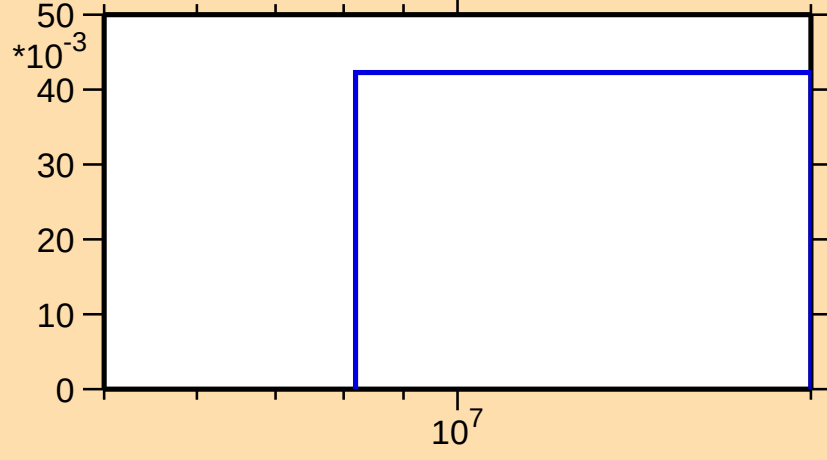
\sigma vs. E for ^{185}\text{Pb}(n,2n)
