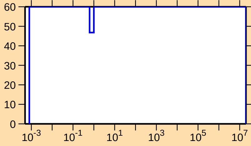
\Delta\sigma/\sigma vs. E for ^{185}\text{Pb}(n,\gamma)
