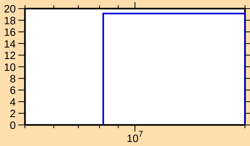
\Delta\sigma/\sigma vs. E for ^{185}\text{Pb}(n,\text{nonel.})
