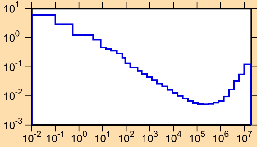
\sigma vs. E for ^{187}\text{Pb}(n,\alpha)
