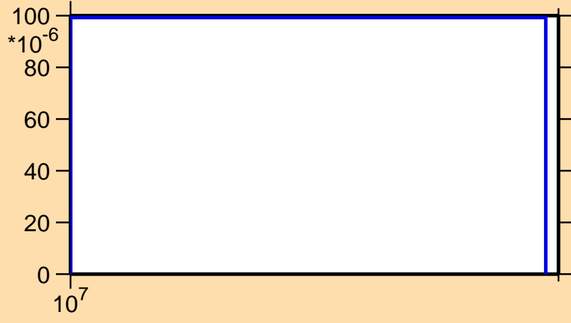
\sigma vs. E for ^{187}\text{Pb}(n,2np)
