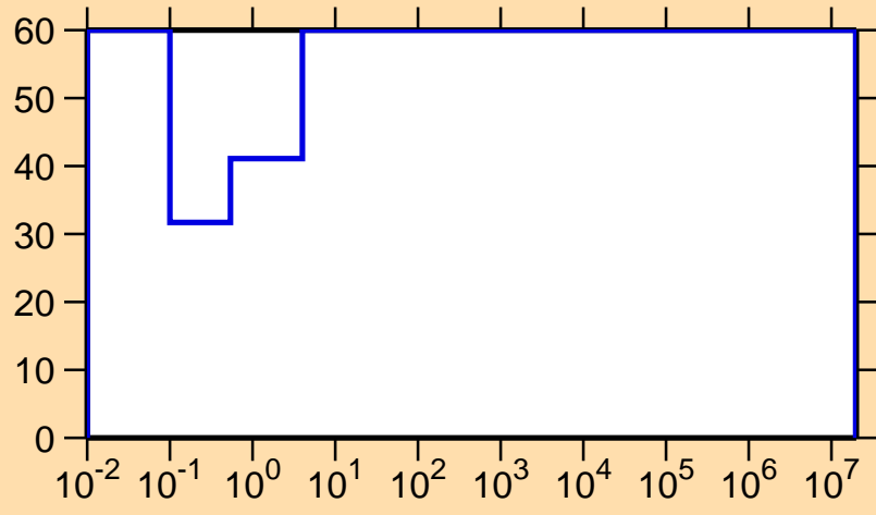
\Delta\sigma/\sigma vs. E for ^{187}\text{Pb}(n,\gamma)
