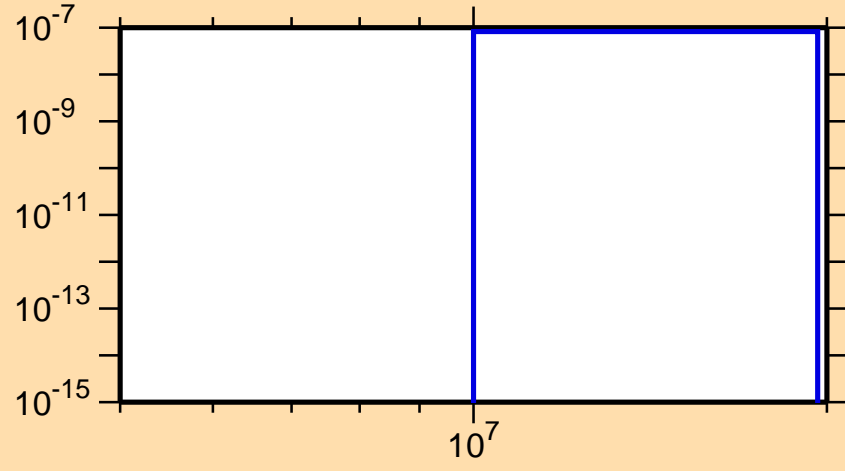
\sigma vs. E for ^{187}\text{Pb}(n,pt)
