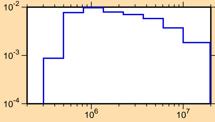
\sigma vs. E for ^{187}\text{Pb}(n,n_2)
