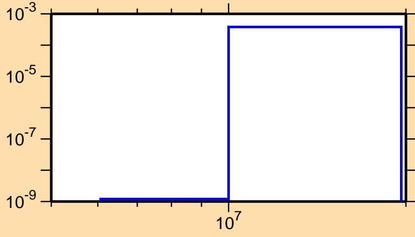
\sigma vs. E for ^{187}\text{Pb}(n,t)
