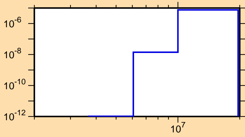
\sigma vs. E for ^{187}\text{Pb}(\text{mt117})
