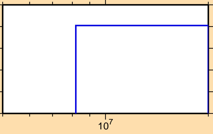
\sigma vs. E for ^{187}\text{Pb}(n,2np)
