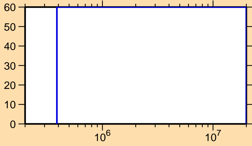
\Delta\sigma/\sigma vs. E for ^{187}\text{Pb}(n,n\text{cont.})
