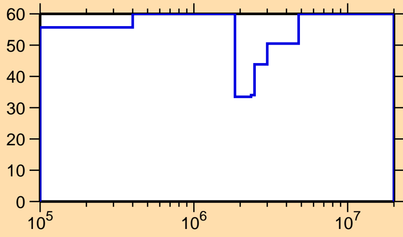
\Delta\sigma/\sigma vs. E for ^{187}\text{Pb}(n, el.)
