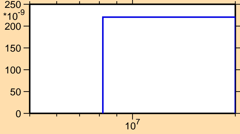
\sigma vs. E for ^{187}\text{Pb}(n,\text{pd})
