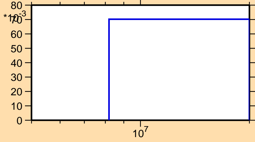
\sigma vs. E for ^{187}\text{Pb}(n,2n)
