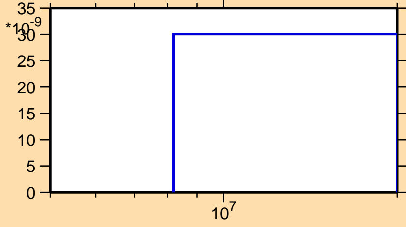
\sigma vs. E for ^{187}\text{Pb}(n,\text{nd})
