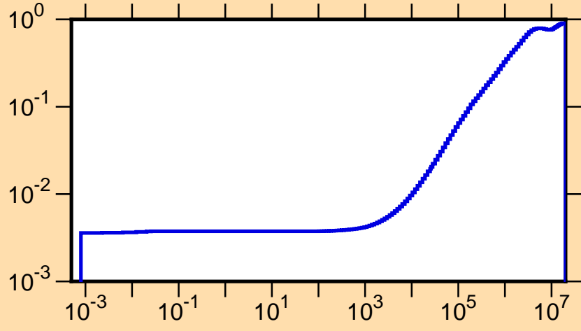
\mu vs. E for ^{188}\text{Pb}(\text{mt251})
