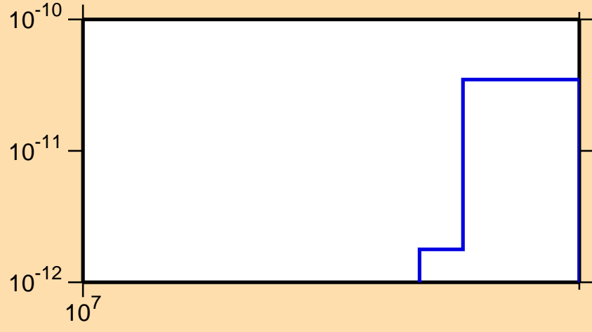
\sigma vs. E for ^{188}\text{Pb} (mt 34)
