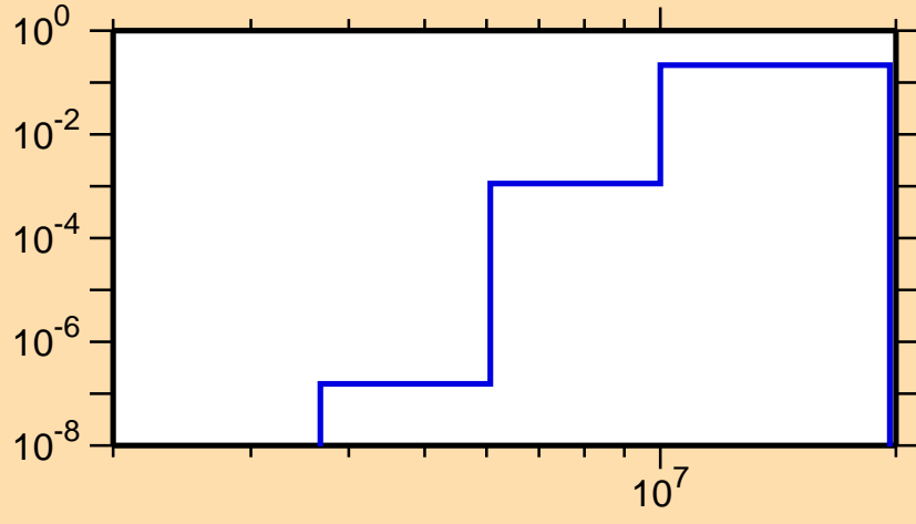
\sigma vs. E for ^{188}\text{Pb}(n,np)
