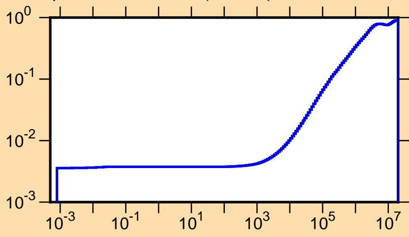
\mu vs. E for ^{189}\text{Pb}(\text{mt251})
