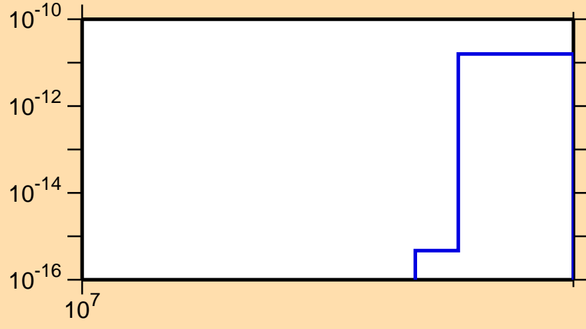
\sigma vs. E for ^{189}\text{Pb}(n,nt)
