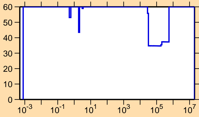
\Delta\sigma/\sigma vs. E for ^{189}\text{Pb}(n,\gamma)
