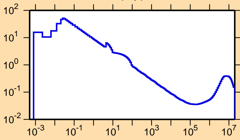
\sigma vs. E for ^{189}\text{Pb}(n,p)
