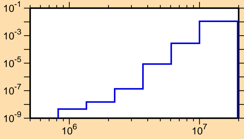
\sigma vs. E for ^{189}\text{Pb}(n,n\alpha)
