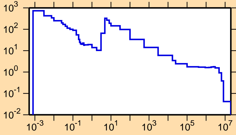
\sigma vs. E for ^{189}\text{Pb}(n,\gamma)
