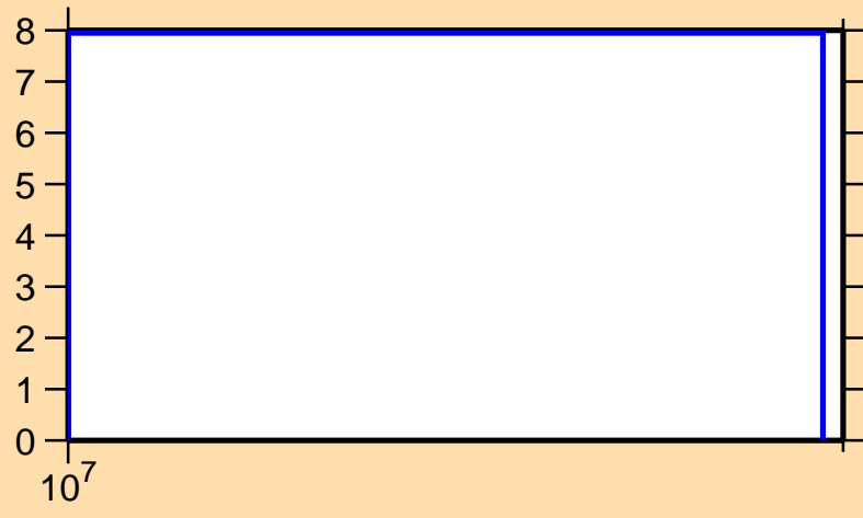
\Delta\sigma/\sigma vs. E for ^{190}\text{Pb}(n,\text{el.})
