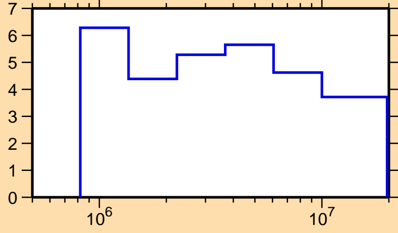
\Delta\sigma/\sigma vs. E for ^{190}\text{Pb}(n, tot.)
