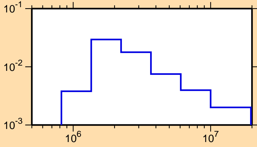
\sigma vs. E for ^{190}\text{Pb}(n,n_3)
