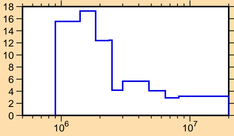
\Delta\sigma/\sigma vs. E for ^{190}\text{Pb}(n,n\text{onel.})
