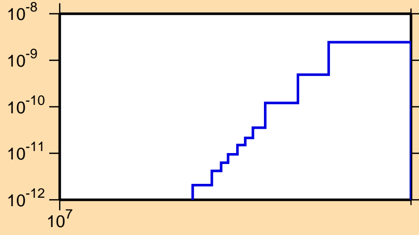
\sigma vs. E for ^{191}\text{Pb}(\text{mt117})
