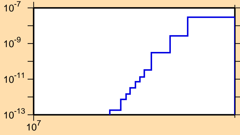
\sigma vs. E for ^{191}\text{Pb}(n,\text{pt})
