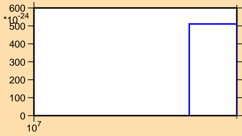
\sigma vs. E for ^{191}\text{Pb}(\text{mt } 11)
