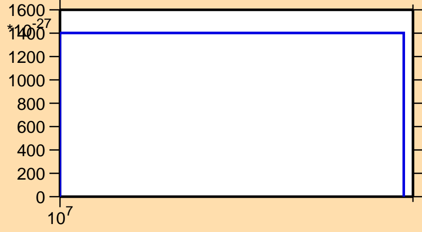
\sigma vs. E for ^{191}\text{Pb} (mt 11)
