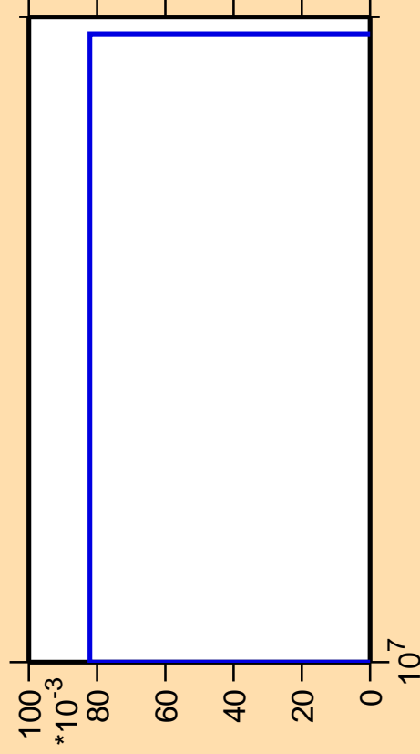
\Delta\sigma/\sigma vs. E for ^{191}\text{Pb}(n,3n\alpha)
