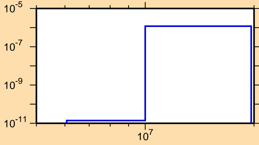
\sigma vs. E for ^{191}\text{Pb}(n,\text{He3})
