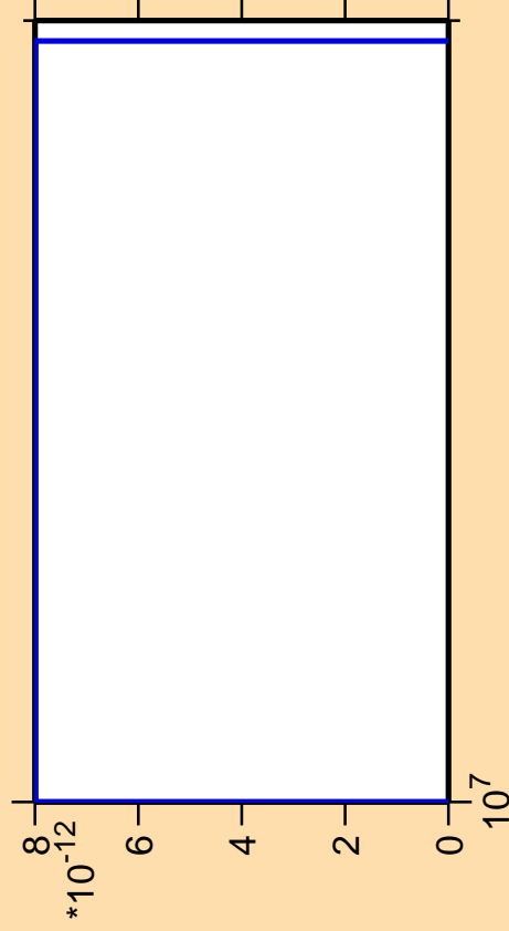
\Delta\sigma/\sigma vs. E for ^{191}\text{Pb} (mt 11)
