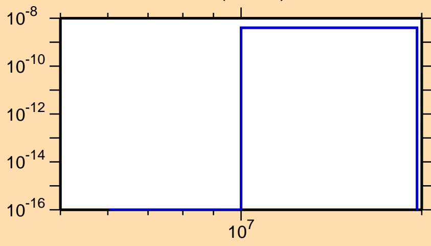
\sigma vs. E for ^{191}\text{Pb}(\text{mt } 45)
