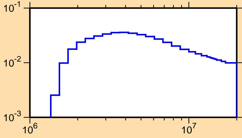
\sigma vs. E for ^{192}\text{Pb}(n,n_4)
