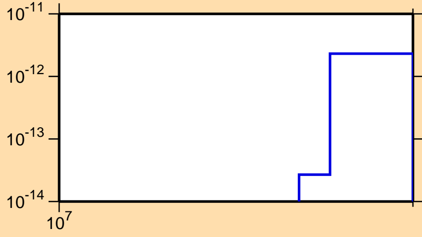
\sigma vs. E for ^{192}\text{Pb}(\text{mt } 34)
