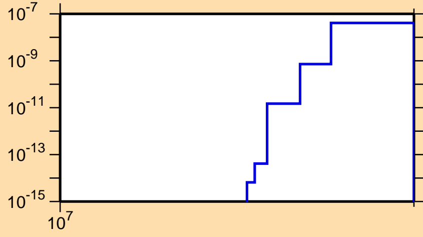
\sigma vs. E for ^{192}\text{Pb}(n,\text{nd})
