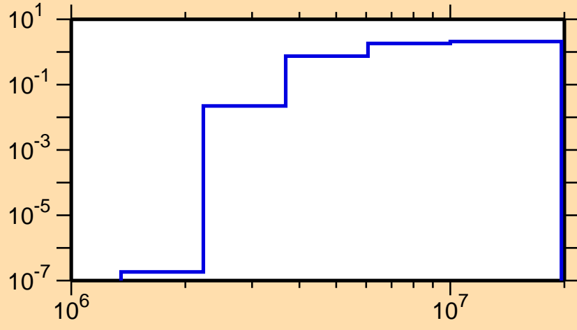
\sigma vs. E for ^{192}\text{Pb}(n,n\text{cont.})
