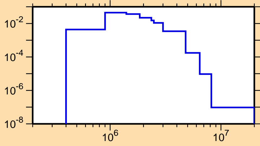
\sigma vs. E for ^{192}\text{Pb}(n,n_1)
