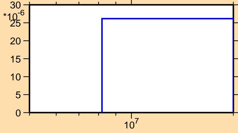
\sigma vs. E for ^{192}\text{Pb}(n,t)
