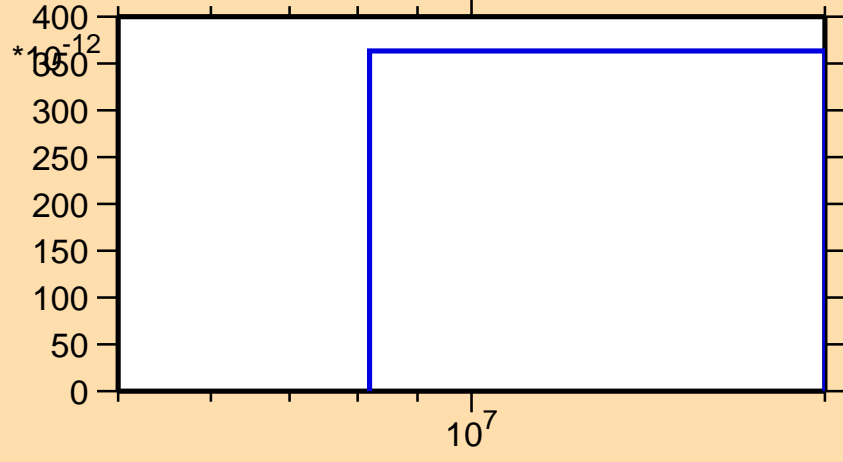
\sigma vs. E for ^{192}\text{Pb}(n,nd)
