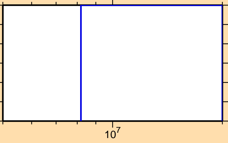
\sigma vs. E for ^{192}\text{Pb}(n,\text{pt})
