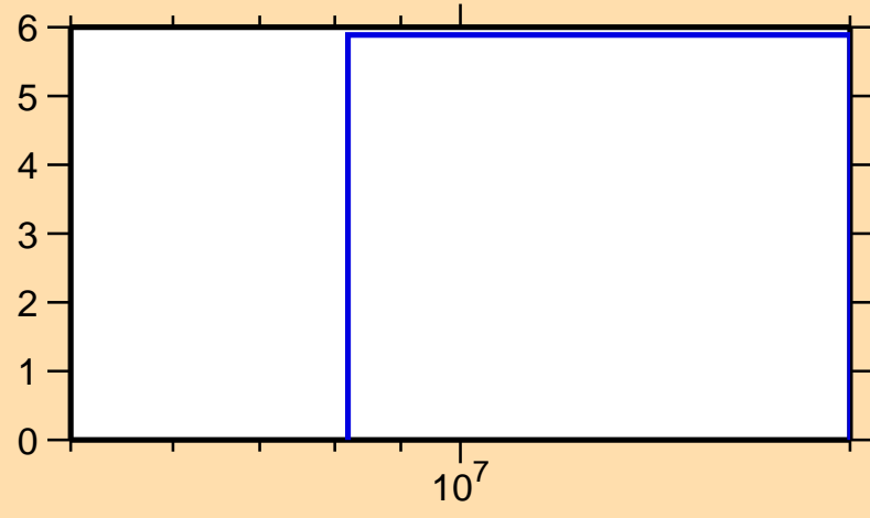
\Delta\sigma/\sigma vs. E for ^{192}\text{Pb}(n,\text{nonel.})
