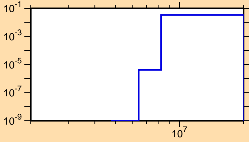
\sigma vs. E for ^{192}\text{Pb}(n,np)
