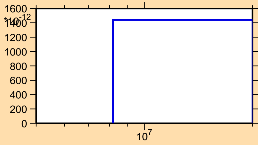
\sigma vs. E for ^{192}\text{Pb}(\text{mt } 45)
