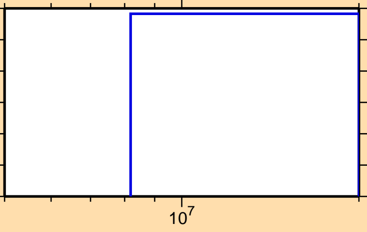
\sigma vs. E for ^{192}\text{Pb}(n,2n\alpha)
