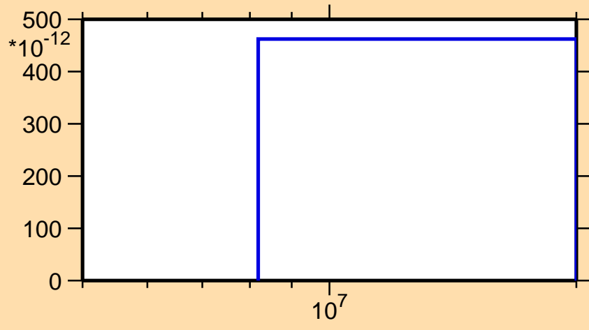
\sigma vs. E for ^{192}\text{Pb}(n,\text{pd})
