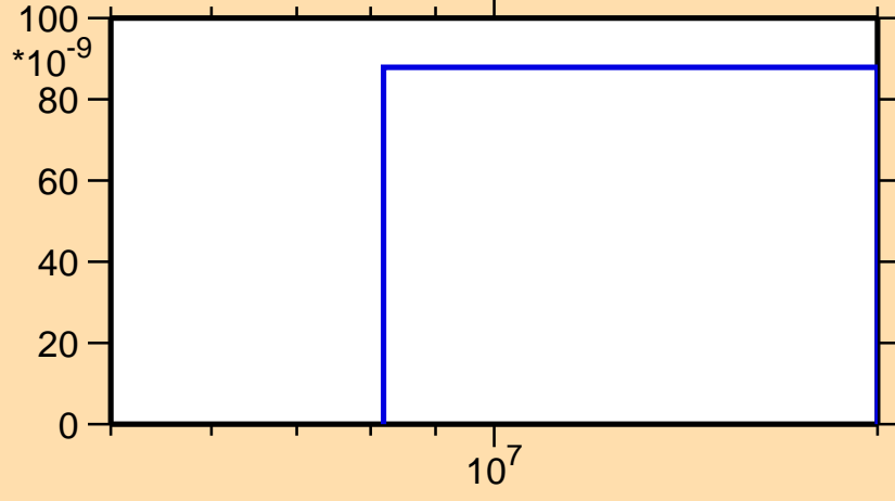
\sigma vs. E for ^{192}\text{Pb}(n,\text{He}3)
