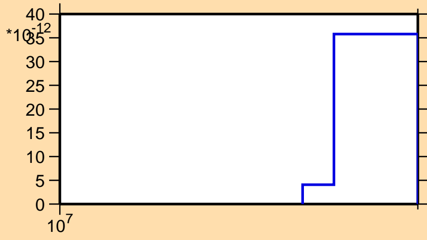
\sigma vs. E for ^{193}\text{Pb}(\text{mt117})
