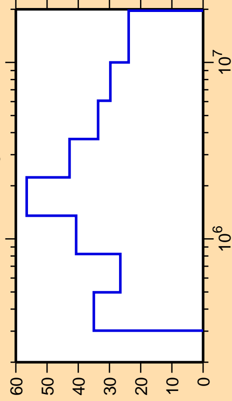
\Delta\sigma/\sigma vs. E for ^{193}\text{Pb}(n,n_3)
