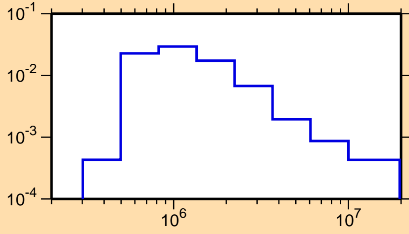
\sigma vs. E for ^{193}\text{Pb}(n,n_3)
