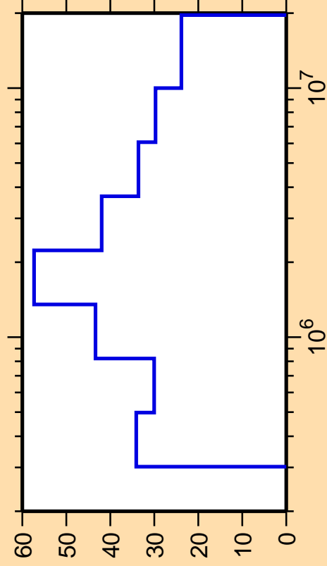
\Delta\sigma/\sigma vs. E for ^{193}\text{Pb}(n,n_2)
