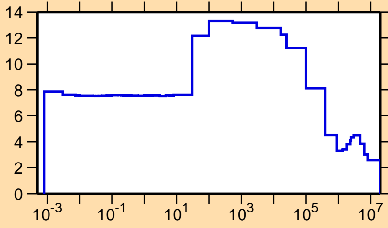
\sigma vs. E for ^{193}\text{Pb}(n,\text{el.})
