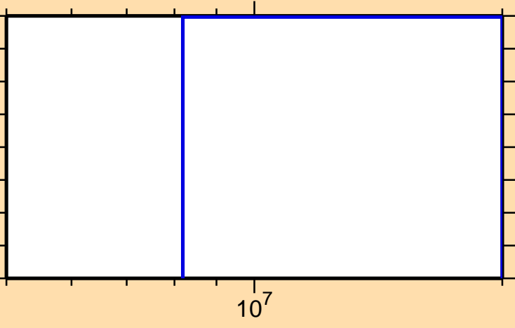
\sigma vs. E for ^{193}\text{Pb}(\text{mt } 45)
